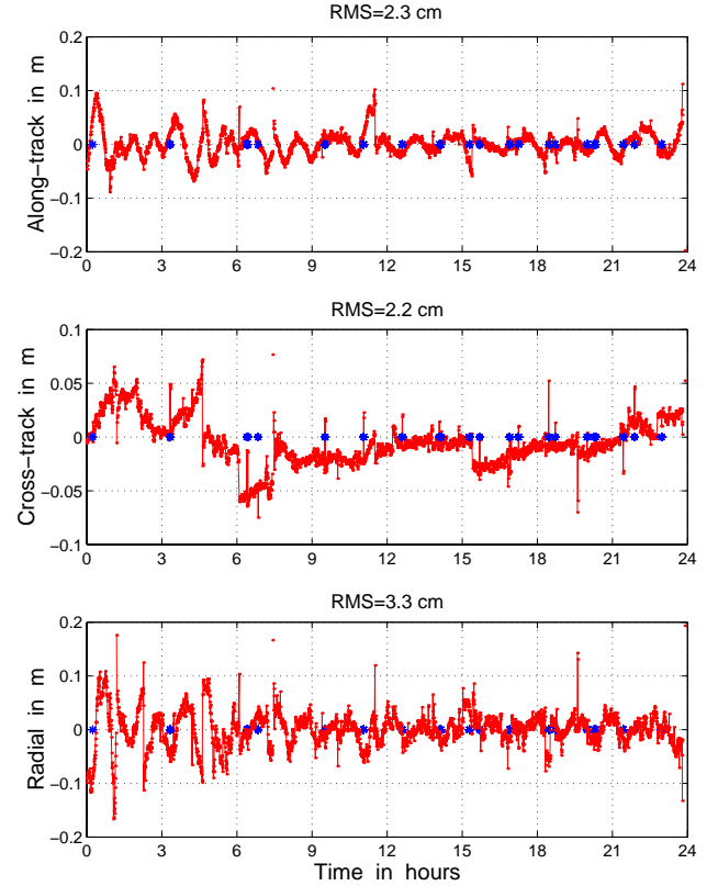
Fig. 11. Zero-diff. kinematic orbit compared to dynamic orbit, day 202/2002, stars are epochs with missing attitude information.
