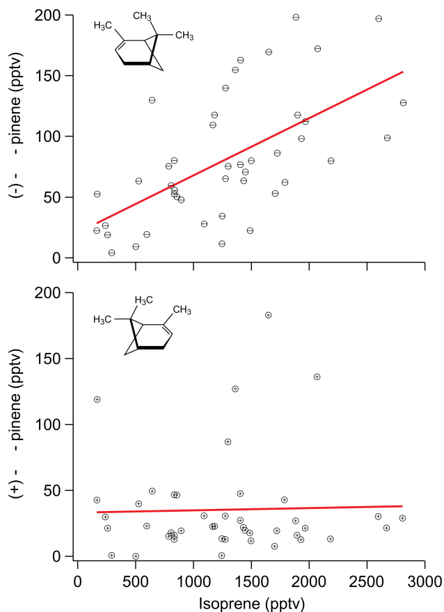
Fig. 6. Correlations of (-)\alpha -pinene and (+)\alpha -pinene with isoprene. The data presented were taken by aircraft over the forest between 0–2 km. The enantiomeric structures of (-)\alpha -pinene and (+)\alpha -pinene are inserted top left in each panel.
