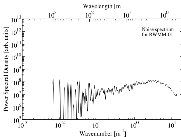
Fig. 1. Wavelet power spectral density for the RWMM-01 PIP directly before launch, while the payload was at the launch pad. For the wavelength, a velocity of 560 m/s is assumed, which corresponds to an altitude of 62.6 km for this payload.
