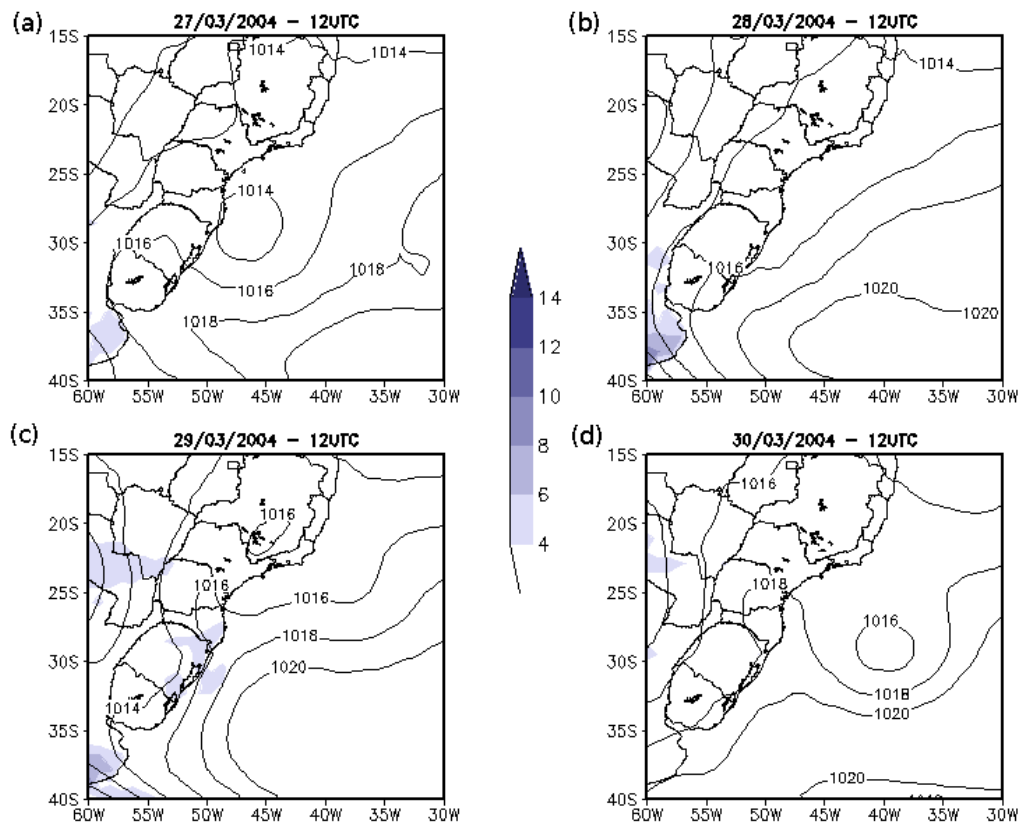
Fig. 5. SLP (solid lines, in \text{hPa} ) and V10m (shading in \text{ms}^{-1} ) 24-h CPTEC/AGCM forecasts of the valid for: (a) 03/27, (b) 03/28, (c) 03/29 and (d) 03/30 at 12:00 UTC.
