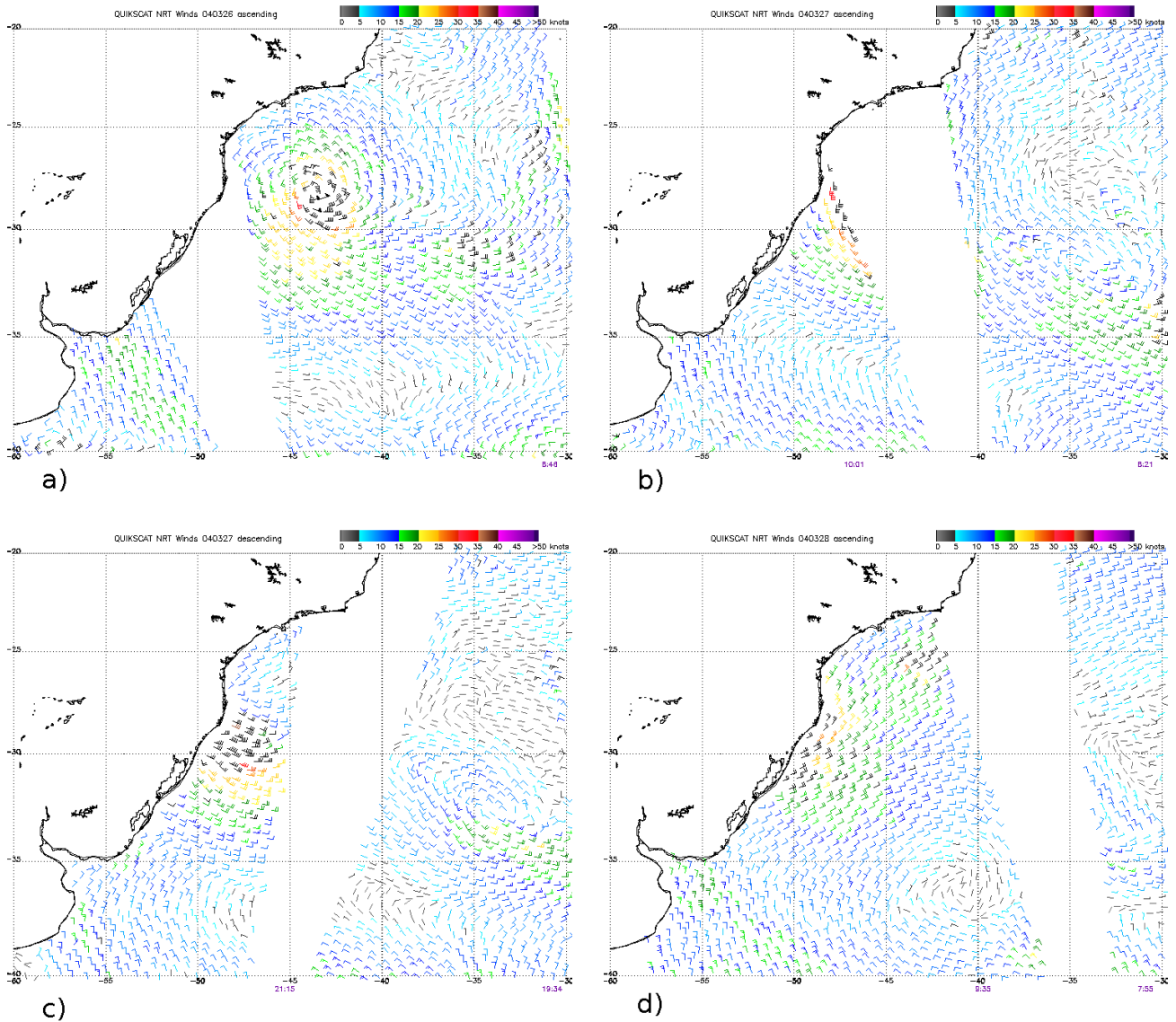
Fig. 3. QuikSCAT fields during: (a) 03/26, ascending passage; (b) 03/27, ascending passage; (c) 03/27, descending passage; (d) 03/28, ascending passage. Wind in knots and black bars indicate possible rain contamination. Team (2007)
