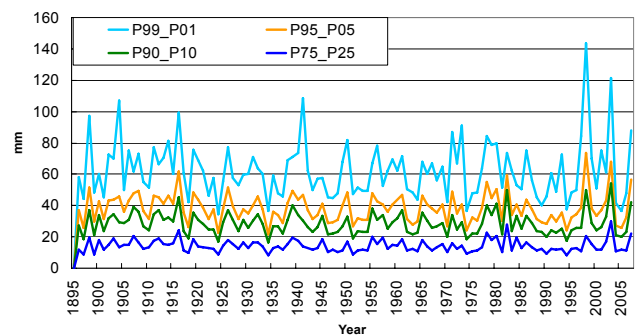
Fig. 9. Long-term fluctuations of values not exceeded by annual maximum of daily precipitation totals for 98, 90, 80 and 50%-part of area of CR. (labeled as P99_P01, P95_P05, P90_P10 and P75_P25). Period 1895–006.
