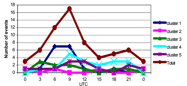
Fig. 5. The number of snow events versus the first hour of their report for each cluster.
