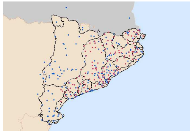
Fig. 4. Distribution of the 313 rainfall stations used in the present work. Red dots are the stations used in the analogous methods and blue ones are the other stations used for developing observed rainfall charts.
