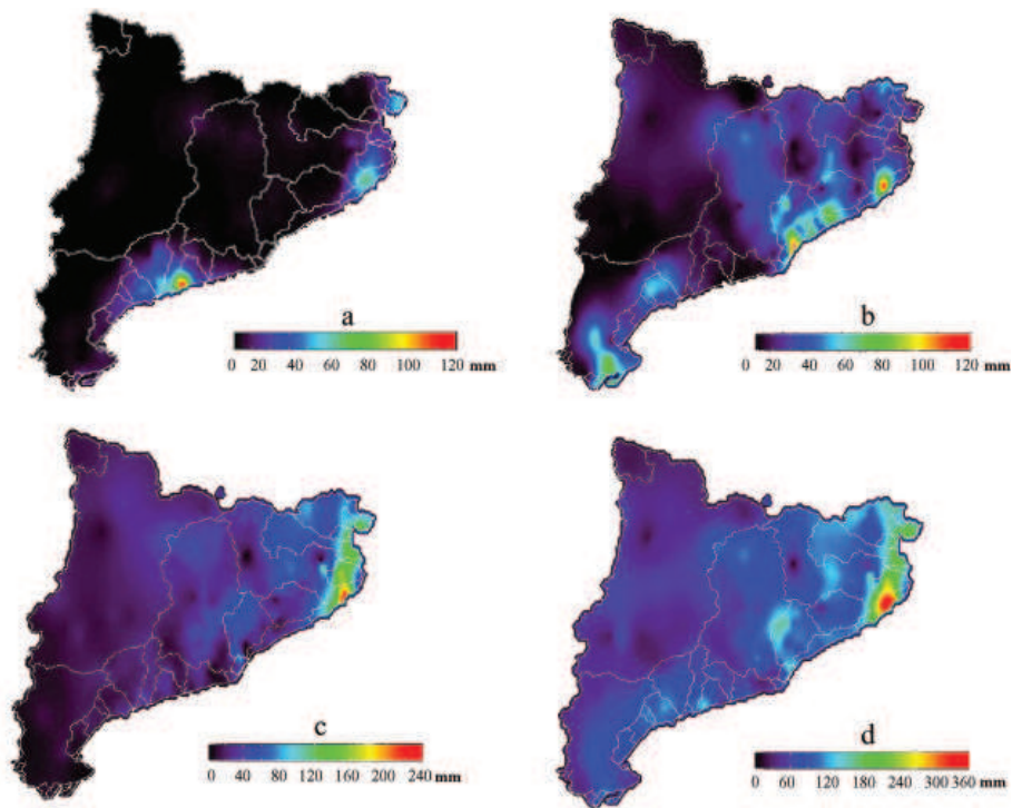
Fig. 1. Recorded precipitation from 00:00 to 24:00 UTC over Catalonia on 11 October 2005 (a), 12 October 2005 (b), 13 October 2005 (c) and total accumulated precipitation from 11 October 2005 at 00:00 UTC to 16 October 2005 at 00:00 UTC (d). Data obtained from 313 stations.
