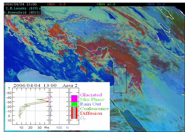
Fig. 11. As Fig. 9 only for 4 April 2006, 13:00 GMT area 2; the microphysical zones show here very deep diffusional growth zone (~25°C), followed by shallow mixed phase zone (~12°C) and glaciation zone (~15°C). D_{15} shows extremely continental values of ~27°C, as those of clouds in heavy smoke (Lensky and Drori, 2007). A tornado followed shortly after in this area.
