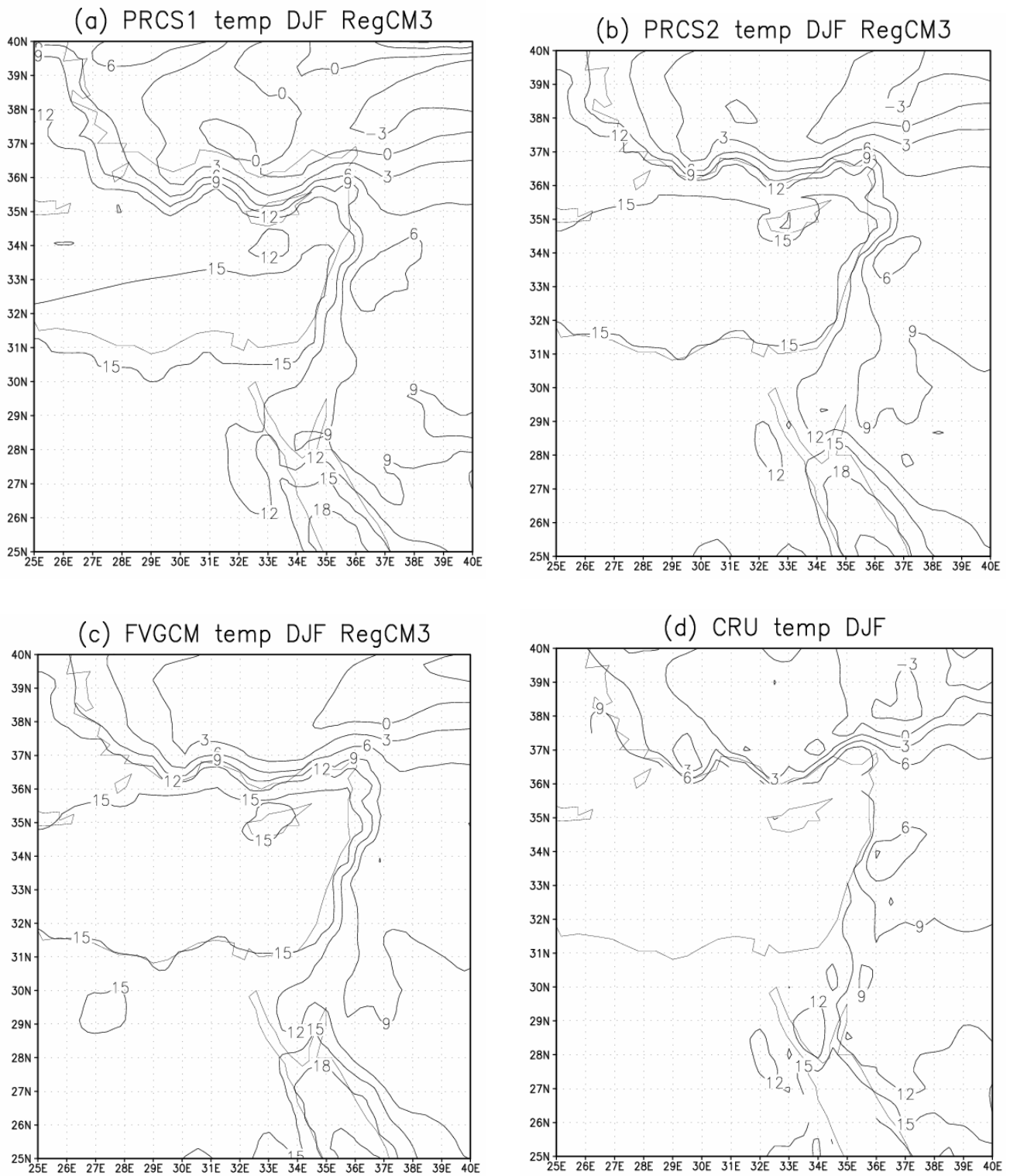
Fig. 2. December-January-February long-term mean near surface air temperature (°C) produced in (a) PRCS1, (b) PRCS2, (c) FVGCM experiments and (d) CRU data.
