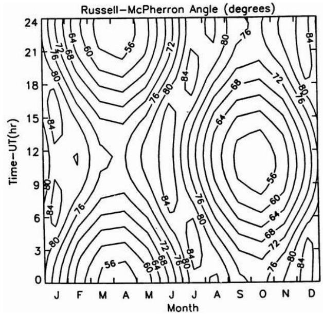
Fig. 2. UT/seasonal variations of the angle \varphi , controlling parameter in the Russell-McPherron mechanism, according to the data of Cliver et al. (2000).
