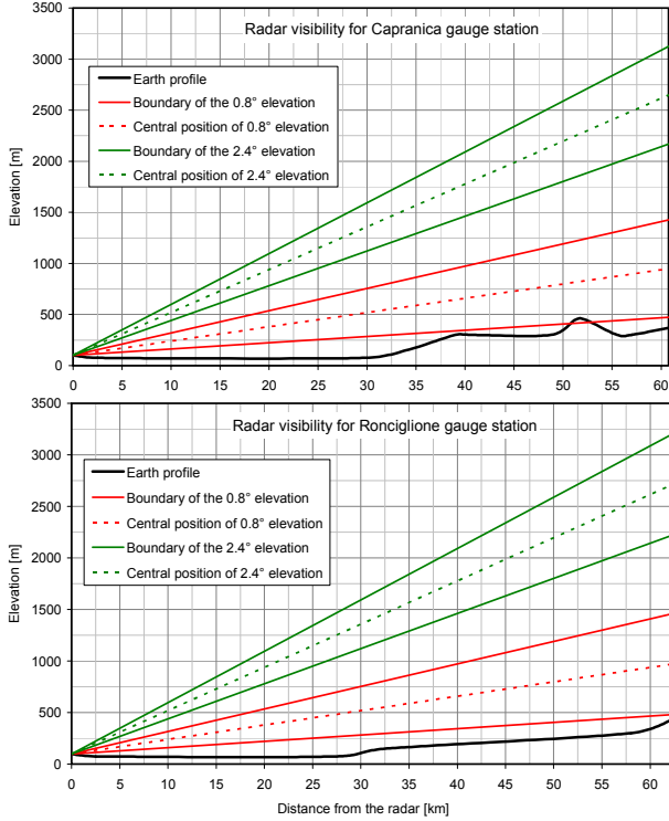
Fig. 1. Profile between the radar and Capranica and Ronciglione rain gauge stations. It is shown the Earth profile (black line) the central position of the beam for two different elevation angles (dotted lines) and the beam width for the same elevation angles.
