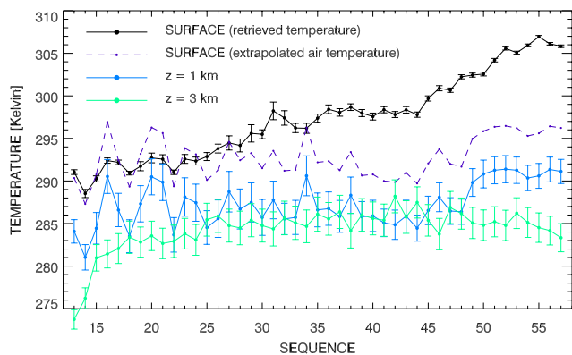
Fig. 8. Time series of temperature values as measured by REFIR at the surface (surface brightness temperature) and at the retrieval altitudes of 1.0 and 3.0 km.
