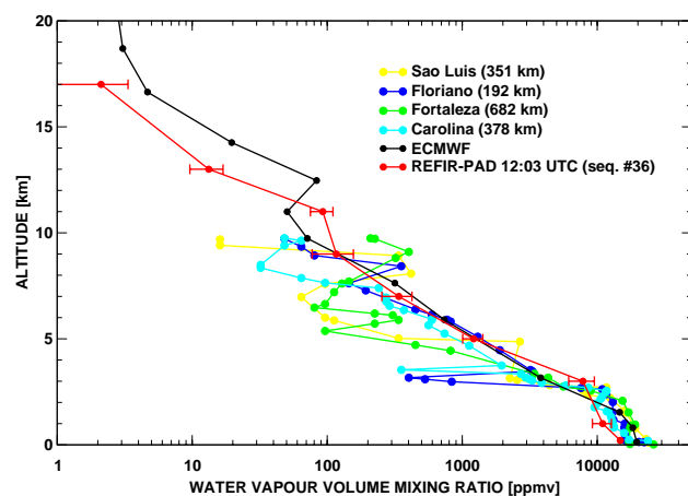
Fig. 3. Retrieval of the water vapour vertical profile (red line) and comparison with the ECMWF profile (black line) and the existing nearby radiosondes (coloured dots). In parenthesis the distance of each radiosounding station from REFIR-PAD. For best coincidence with radiosoundings the profile for sequence #36 measured around noon UTC is reported.
