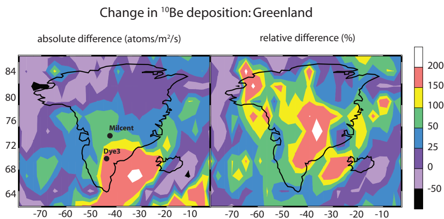
Fig. 9. The change of modeled ^{10}\text{Be} deposition between Maunder Minimum and Present Day in Greenland in absolute (atoms/m 2 /s, left) and relative (% , right) units
