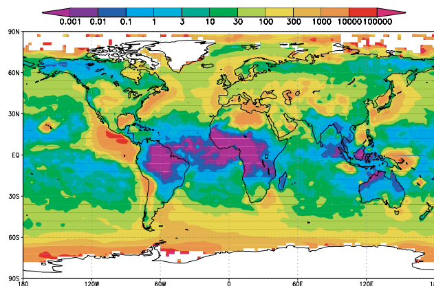
Fig. 4. The ratio of annual mean IMN rates integrated within the lowest 3 km of atmosphere (e.g., the source strength due to IMN, \text{SS}_{\text{IMN}0-3} , \# \text{ cm}^{-2} \text{ day}^{-1} ) to the annual mean rate of emission of primary particles (e.g., source strength due to primary aerosol emission, \text{SS}_{\text{primary}} , \# \text{ cm}^{-2} \text{ day}^{-1} ). The primary aerosols considered in GEOS-Chem, and their corresponding assumed (fixed) sizes (radius), are: dust (4 sizes: 0.7, 1.5, 2.5, 4 \mu\text{m} ), sea salt (3 sizes: 0.732, 5.67 \mu\text{m} , and an ultrafine sea salt mode with a radius of 40 nm), black carbon aerosol (39 nm), and organic carbon particles (70 nm).
