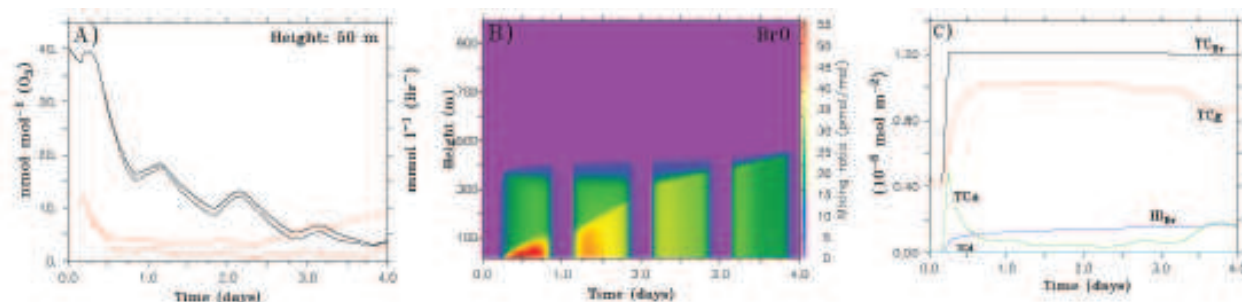
Fig. 16. Run 18 (no-HONO). (A) Comparison between run 18 (dashed lines) and the base run (solid lines) for gas phase O 3 (black lines in nmol mol -1 ) and FF aerosol bromide (red lines in nmol l -1 ) at an altitude of 50 m. (B) BrO in run 18, (C) total bromine budget for run 18.
