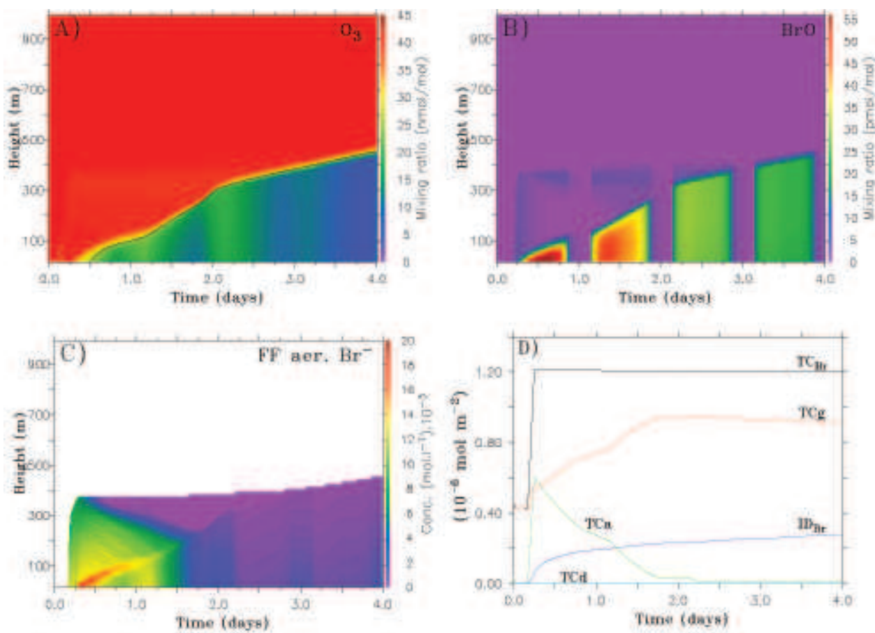
Fig. 11. Run 13. Only 50% of bicarbonate precipitated. (A) O_3 , (B) BrO, (C) FF aerosol bromide, (D) total bromine budget.
