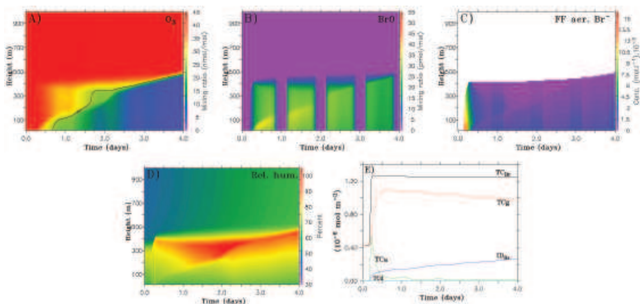
Fig. 10. Run 12. Scaling factor \mu=45 , wind speed =7 \text{ m s}^{-1} . (A) \text{O}_3 , (B) \text{BrO} , (C) FF aerosol bromide, (D) relative humidity, (E) total bromine budget.
