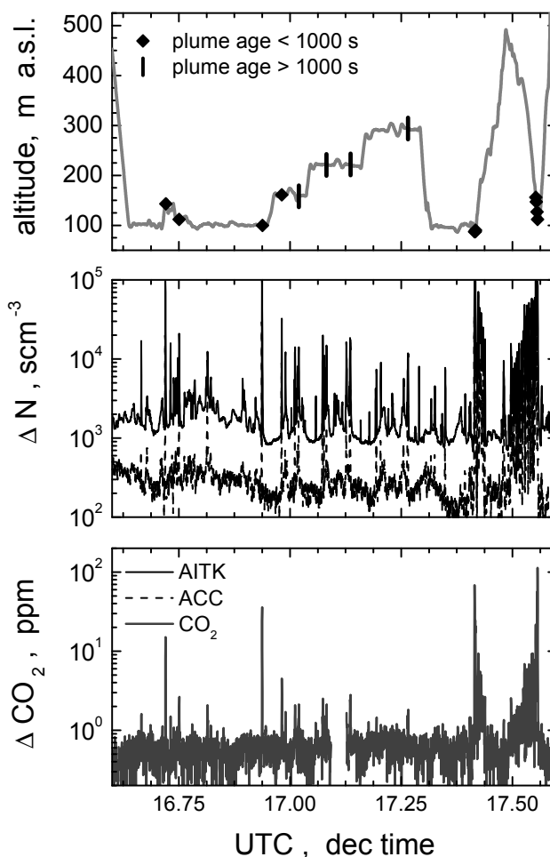
Fig. 7. Time series of flight altitude in m above sea level (a.s.l.): excess number concentration \Delta N for Aitken (AITK, solid line) and accumulation (ACC, dashed line) mode particles, and excess CO 2 ( \Delta\text{CO}_2 , thick gray line) during the Single Plume Study.
