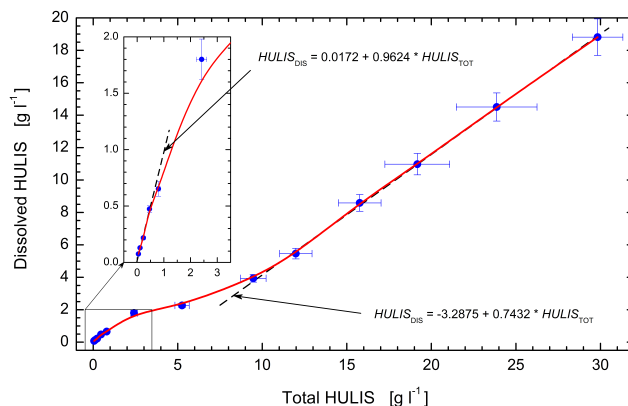
Fig. 2. Dependence of the dissolved HULIS concentration ( \text{HULIS}_{\text{DISS}} ) on the total HULIS concentration ( \text{HULIS}_{\text{TOT}} ) in aqueous samples. The range of small concentrations is also displayed in an insert. The connecting curves represent eye guides only. The limiting linear lines (dashed lines) and their analytical expressions are also shown.
