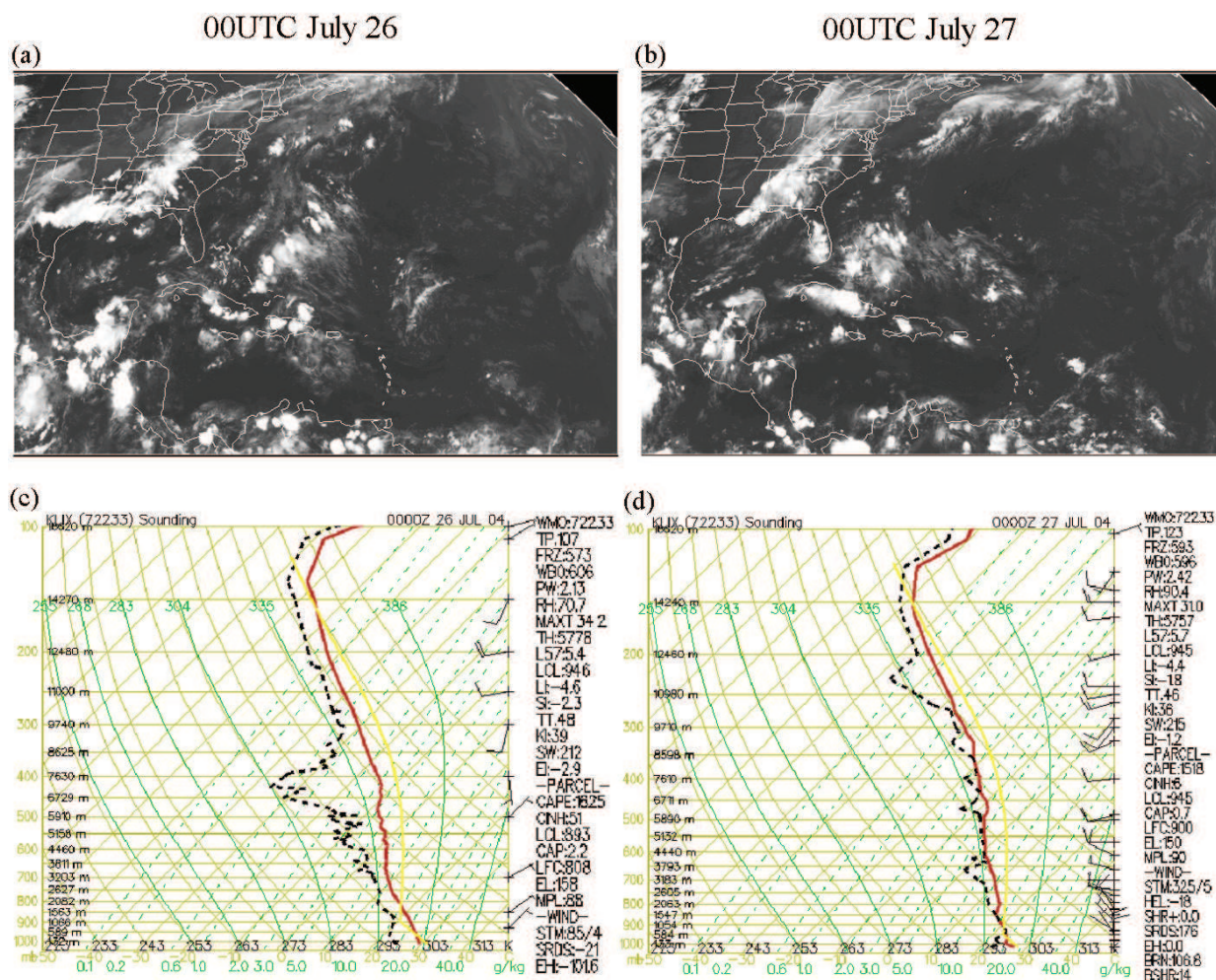
Fig. 3. GOES infrared images (a and b), and skew T and log P diagram (c and d) at the Slidell, Louisiana ( 30.33^{\circ} N and 89.82^{\circ} W) for 00:00 UTC 26 July 2004 and 00:00 UTC 27 July 2004.
