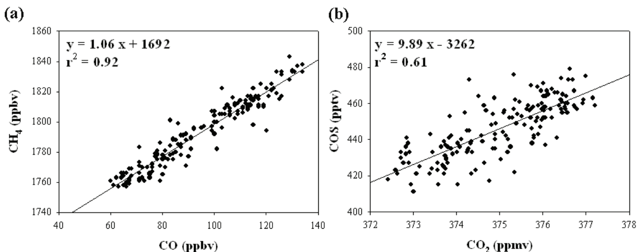
Fig. 8. Correlations (a) between CO and CH 4 , and (b) between CO 2 and COS on flight 13.
