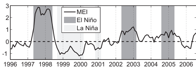
Fig. 2. MEI index time series. Darkgray/lightgray patches represent El Niño/La Niña as identified by NOAA.
