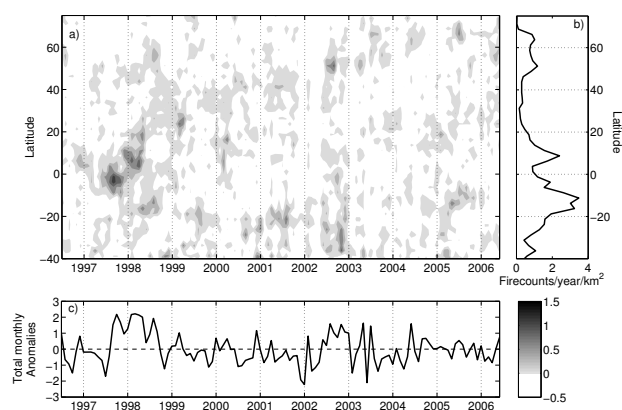
Fig. 1. (a) Time-latitude Hovmöller diagram of monthly deseasonalised fire anomalies (positive anomalies only, scale indicated by the colorbar). (b) Fire counts by latitude (detection/year/km 2 ), corrected by continental surface for each latitudinal band. (c) Monthly anomalies of the total deseasonalised fire counts over the 10 years.
