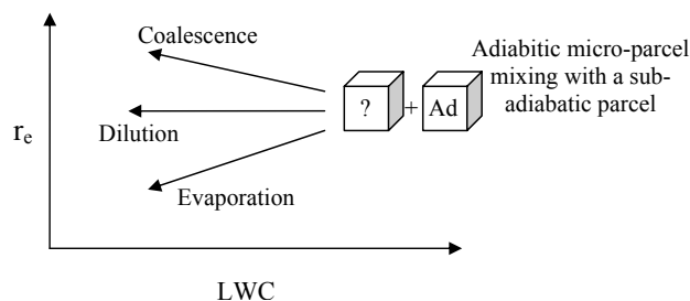
Fig. 15. Schematic illustration of the probable effects of the evaporation, dilution and coalescence processes on the r_e -LWC relation when an adiabatic parcel mixes with another sub-adiabatic parcel. The box marked with “Ad” represents the adiabatic parcel and its location on the r_e -LWC plane is meaningful, while the box marked with a question mark represents the sub-adiabatic parcel and its location on the plane is variable although its LWC has to be smaller than the adiabatic parcel (when there are no falling-from-above precipitation particles). The final location of the newly mixed parcel on the r_e -LWC plane will be determined by the relative importance of the above mentioned processes.
