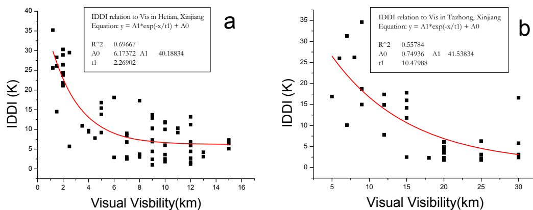
Fig. 6. SDS-IDDl relate to visibility from synoptic visibility data.
