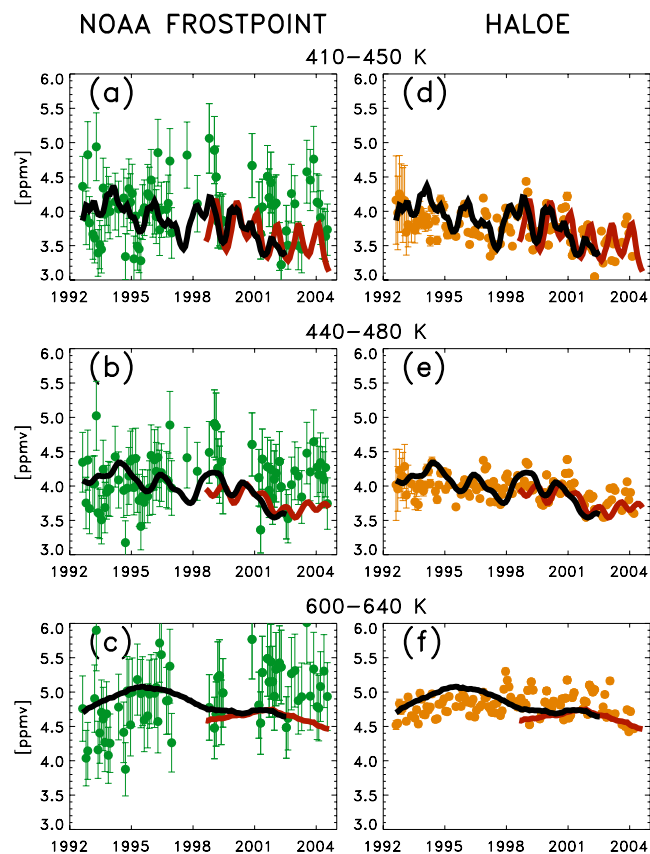
Fig. 8. Observation and model as in Eq. (10) for the layers (a, d) 410–450 K, (b, e) 440–480 K, (c, f) 600–640 K; for NOAA FP (a, b, c) and HALOE (d, e, f). The black line shows the “[H 2 O] e -model” estimate and the red line shows the model estimate using HALOE measurements in the tropics at 400 K (see text). Note that for HALOE, error bars are smaller than the dots, except for low altitudes in the years following the eruption of Mt. Pinatubo.
