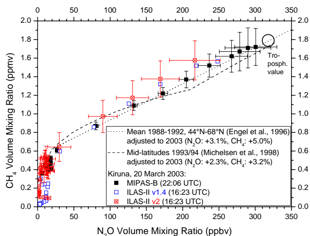
Fig. 4. N 2 O-CH 4 correlations as measured by MIPAS-B and ILAS-II (ILAS-II error bars for CH 4 values less than 0.3 ppmv are omitted for clarity). Trend-corrected reference correlations observed by other instruments (in-situ, Engel et al., 1996, and Atmospheric Trace Molecule Spectroscopy Experiment, Michelsen et al., 1998) are shown for comparison. The Northern Hemispheric tropospheric correlation value of 2003 is marked by a black circle.
