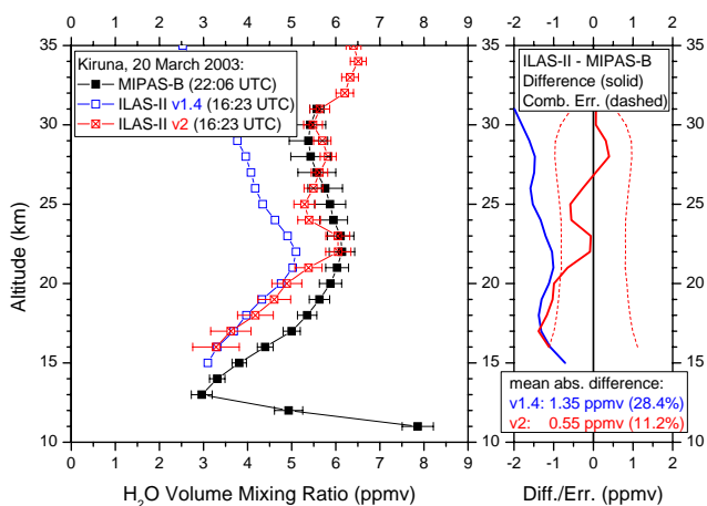
Fig. 5. Comparison of H 2 O profiles as measured by MIPAS-B and ILAS-II. Annotation as per Fig. 1.
