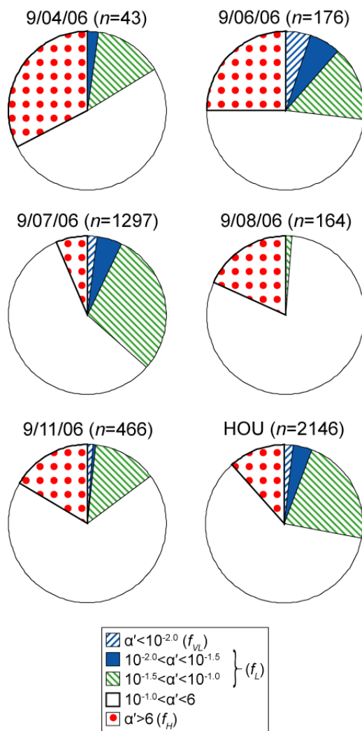
Fig. 8. Summary of CCN \alpha' distributions for each day at HOU, and the total from the site. An \alpha' of 10^{-2.0} is 4\sigma below the mean for ammonium sulfate ( \alpha_{app,AS} ), \alpha'=10^{-1.5} is 3\sigma below \alpha_{app,AS} , \alpha'=10^{-1.0} is 2\sigma below \alpha_{app,AS} , and \alpha'=6 is 1.5\sigma above \alpha_{app,AS} .
