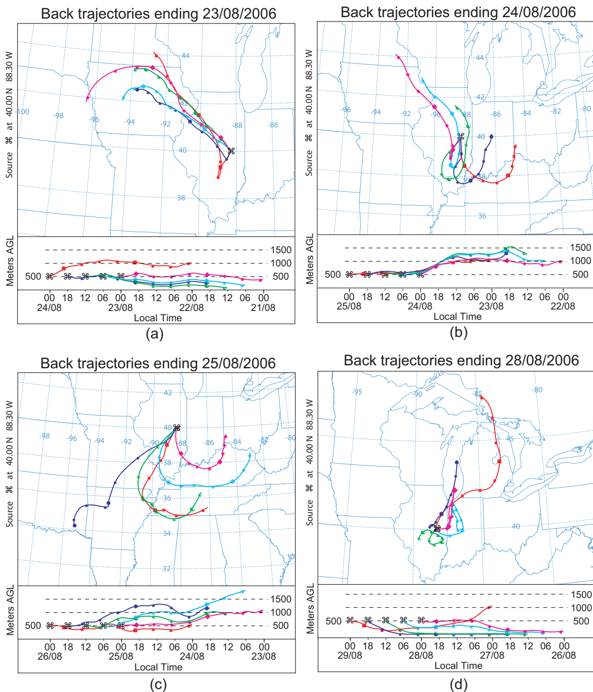
Fig. 12. NOAA HYSPLIT back trajectories ending at the BON site, ending on (a) 23/08/2006, (b) 24/08/2006, (c) 25/08/2006, and (d) 28/08/2006.
