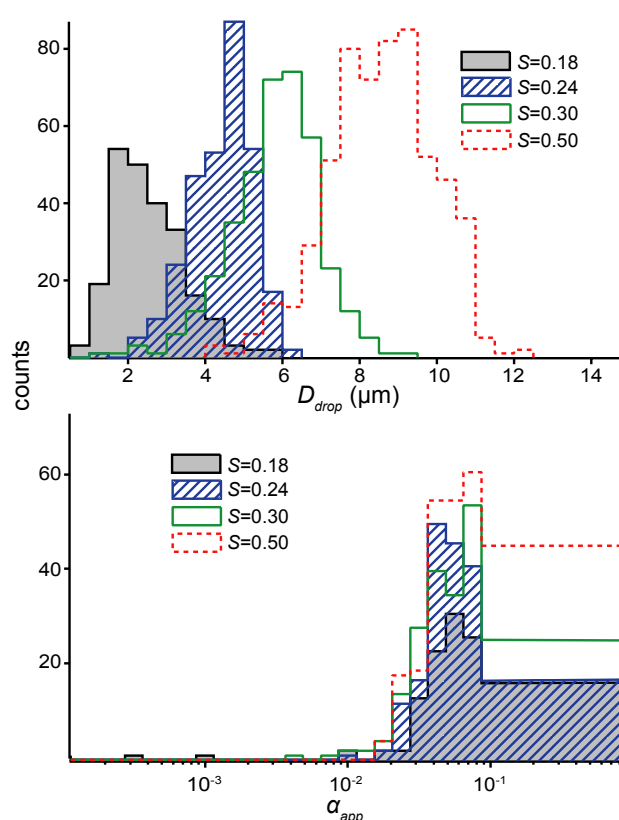
Fig. 4. D and \alpha_{\text{app}} distributions after 30 s of condensational growth at 4 different supersaturations on lab-generated ammonium sulfate particles.
