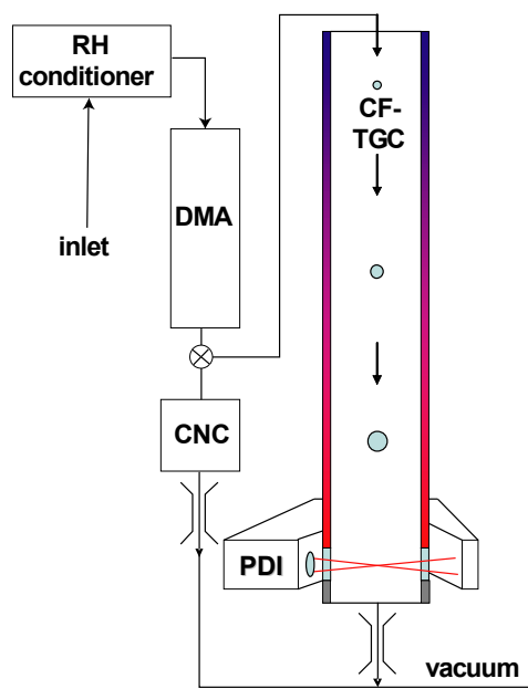
Fig. 2. Experimental schematic.
