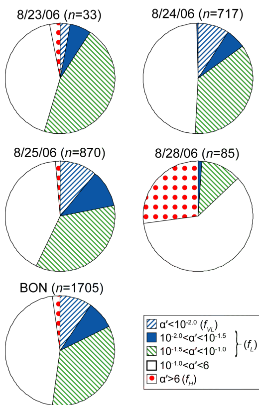
Fig. 7. Summary of CCN \alpha' distributions for each day at BON, and the total from the site. An \alpha' of 10^{-2.0} is 4\sigma below the mean for ammonium sulfate ( \alpha_{app,AS} ), \alpha'=10^{-1.5} is 3\sigma below \alpha_{app,AS} , \alpha'=10^{-1.0} is 2\sigma below \alpha_{app,AS} , and \alpha'=6 is 1.5\sigma above \alpha_{app,AS} .
