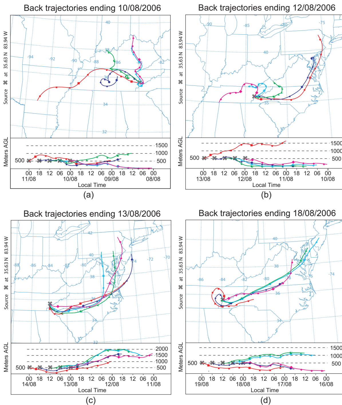
Fig. 13. NOAA HYSPLIT back trajectories ending at the GSM site, ending on (a) 10/08/2006, (b) 12/08/2006, (c) 13/08/2006, and (d) 18/08/2006.
