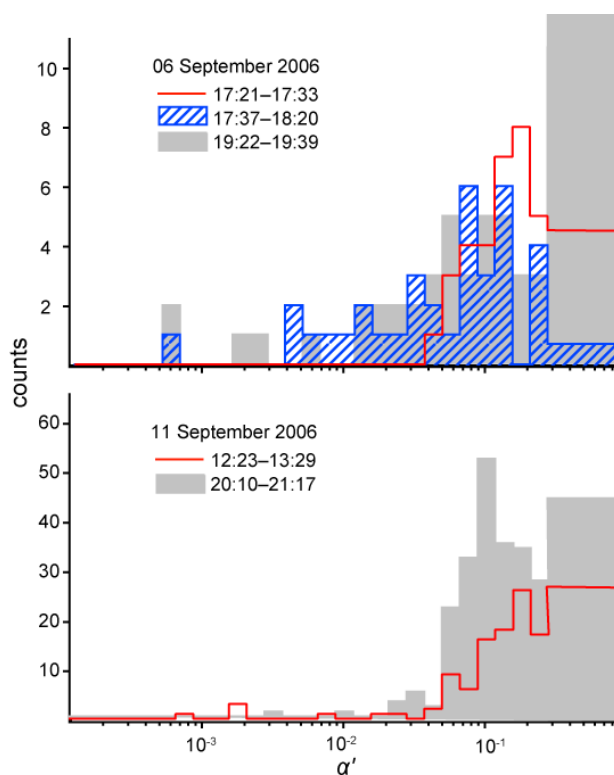
Fig. 11. \alpha' distributions for various periods on two days from HOU.
