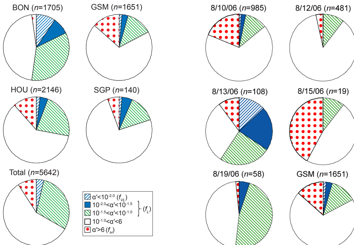
Fig. 5. Summary of CCN \alpha' distributions at each site, and the total of all four sites. An \alpha' of 10^{-2.0} is 4\sigma below the mean for ammonium sulfate ( \alpha_{\text{app,AS}} ), \alpha'=10^{-1.5} is 3\sigma below \alpha_{\text{app,AS}} , \alpha'=10^{-1.0} is 2\sigma below \alpha_{\text{app,AS}} , and \alpha'=6 is 1.5\sigma above \alpha_{\text{app,AS}} .
