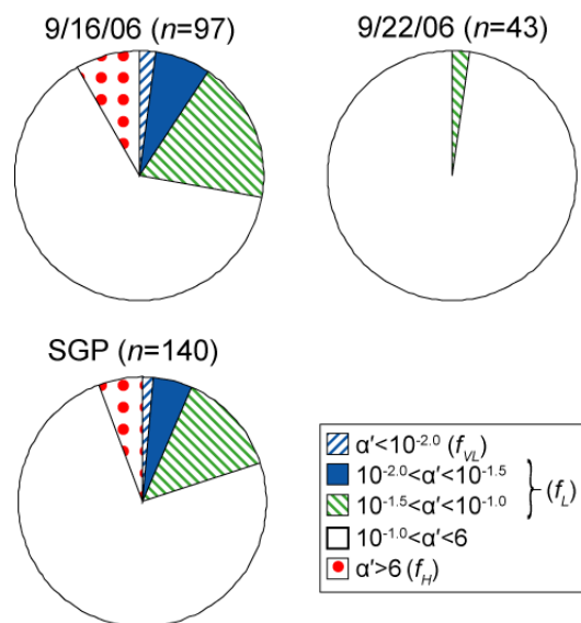
Fig. 9. Summary of CCN \alpha' distributions for both days at SGP, and the total from the site. An \alpha' of 10^{-2.0} is 4\sigma below the mean for ammonium sulfate ( \alpha_{\text{app,AS}} ), \alpha'=10^{-1.5} is 3\sigma below \alpha_{\text{app,AS}} , \alpha'=10^{-1.0} is 2\sigma below \alpha_{\text{app,AS}} , and \alpha'=6 is 1.5\sigma above \alpha_{\text{app,AS}} .
