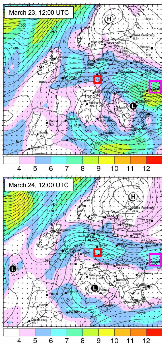
Fig. 3. Charts of selevel pressure (hPa) and horizontal surface wind speeds in Beaufort (colour code) on 23 and 24 March 2007, 12:00 UTC respectively. The charts were produced using the MM5 model and selected from the EURAD products offered by the University of Cologne, Germany ( http://www.eurad.uni-koeln.de ). Squares indicate the source region of the dust plume (magenta) and the region of the key measurements in Saxony, Germany (red).
