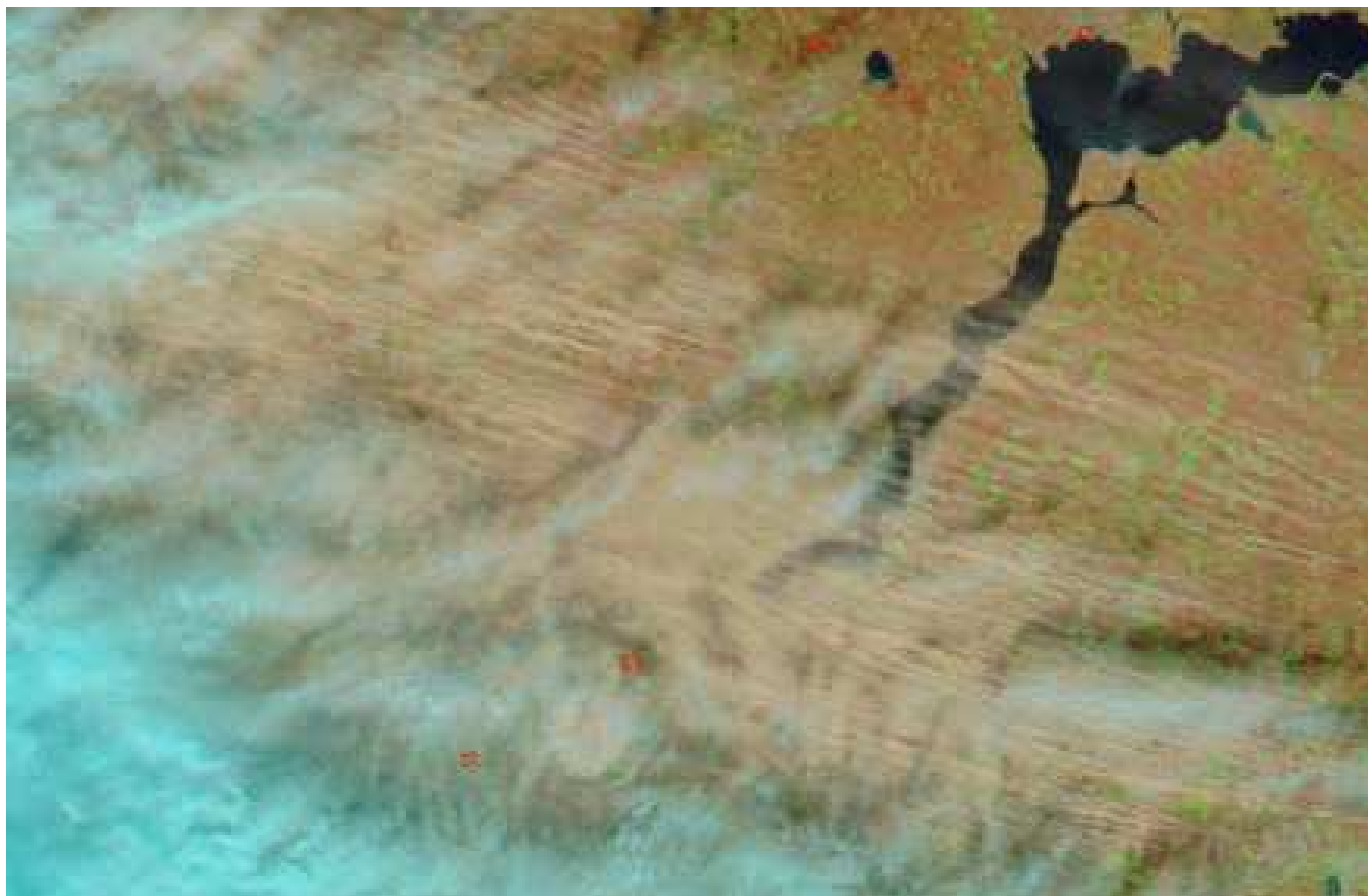
Fig. 2. The MODIS-Aqua composite image of Southern Ukraine on 23 March 2007, 10:50 UTC reveals the large scale emission of agricultural dust. The reservoir lake of Kakhovskaya on the Dnieper River can be seen in dark blue, ice clouds in light blue. Red boxes indicate thermal anomalies, caused in most cases by fire or even flares from a gas well. The dimensions of the area shown is 210 \times 146 km.
