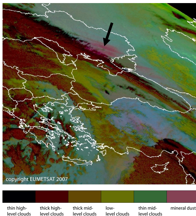
Fig. 1. Dust source activation on 23 March 11:00 UTC over the southern Ukraine (arrow). The image shows MSG dust index images, based on BTD using the 8.7 μm, 10.8 μm and 12.0 μm wavelength bands of the SEVIRI instrument.
