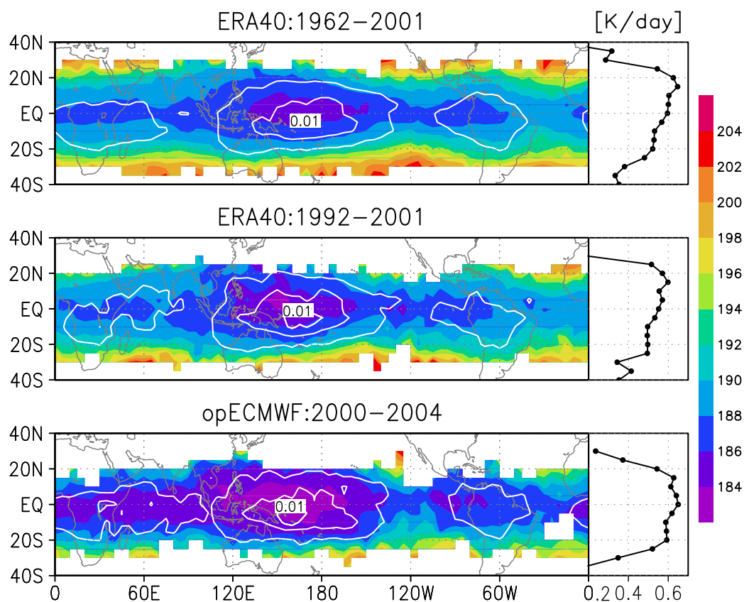
Fig. 3. DJF long-term climatology; Left: LCP temperature [K] (color) and the density of LCPs (white contours); Right: Zonal mean \hat{Q}_{LCP} [K/day]. Top panel: 1962/1963–2001/2002 ERA40 data; middle panel: 1992/1993–2001/2002 ERA40 data; lower panel: opECMWF data from 2000/2001–2004/2005. Contour intervals for the density are 0.001, 0.005 and 0.01 per 5^\circ \times 5^\circ grid.
