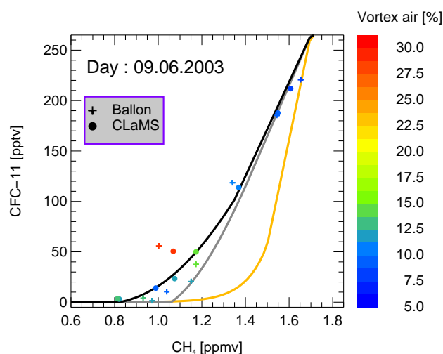
Fig. 2. \text{CH}_4/\text{CFC-11} relation colored with the CLaMS vortex tracer observed on 9 June 2003 (crosses) and the corresponding simulation (filled circles). A clear signature of air masses with about 30% vortex air indicates vortex remnants in the range between 500 and 600 K.
