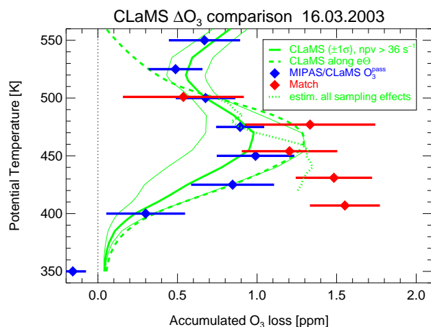
Fig. 5. Vortex average accumulated ozone losses on 16 March versus potential temperatures for different methods. Solid lines correspond to CLaMS results, dashed to ozone loss rates integrated along e\Theta surfaces. Other ozone loss estimates are also included. The Match results are shown with red symbols. Estimates from MIPAS data and CLaMS passive ozone are shown with blue symbols. The dotted line is an estimate that includes the sampling effects as discussed in the text.
