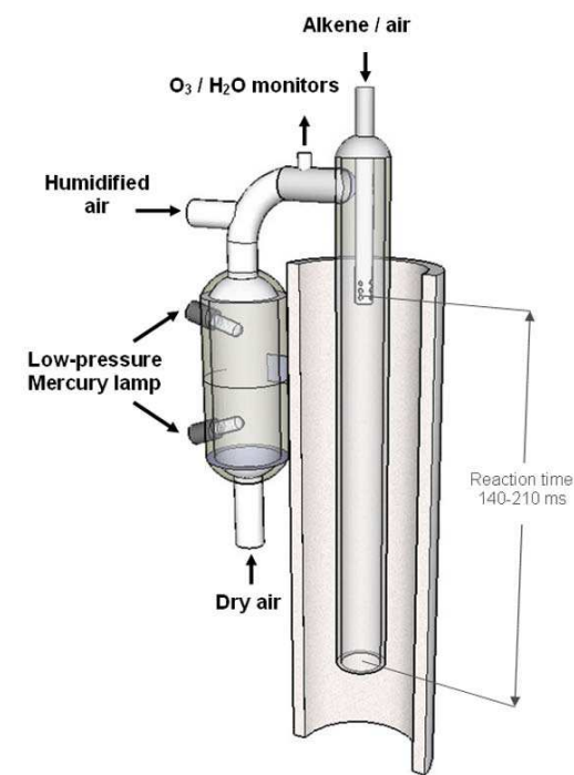
Fig. 4. Schematic of the calibrator based on the steady-state \text{O}_3 -alkene technique.
