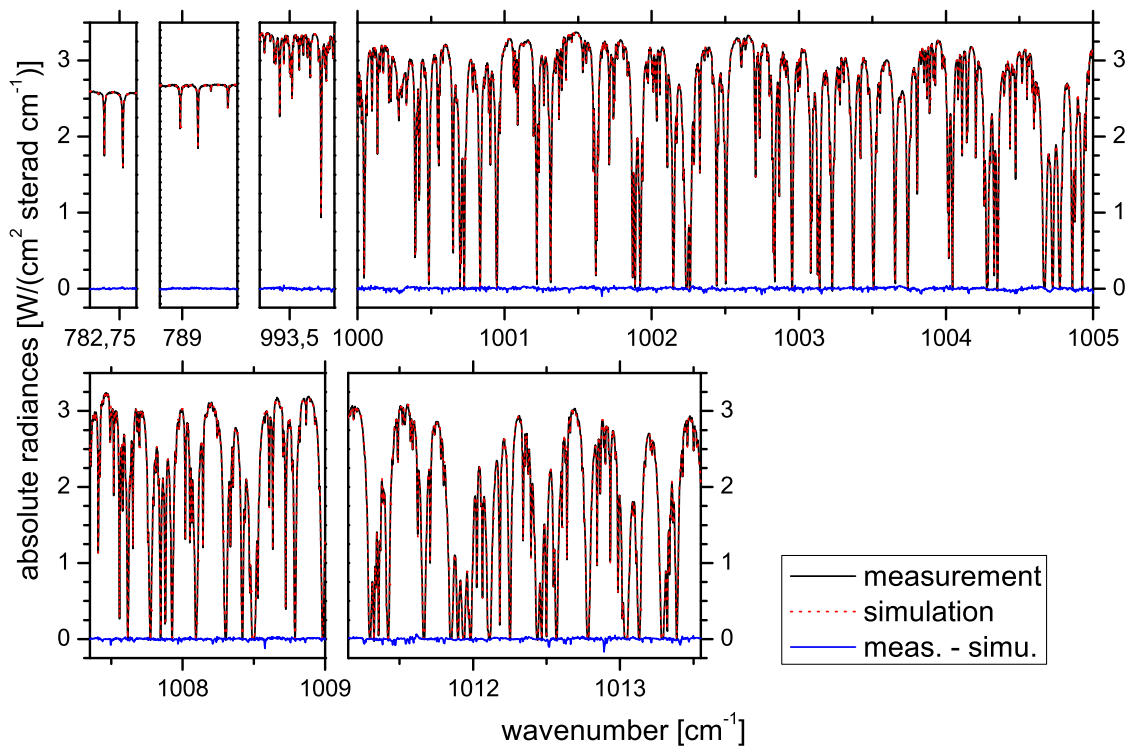
Fig. 1. Spectral windows applied. Plotted is the situation for a real measurement taken on 22nd of January 2005 (solar elevation angle 32.2^\circ ); black line: measured spectrum; red line: simulated spectrum; blue line: difference between simulation and measurement.
