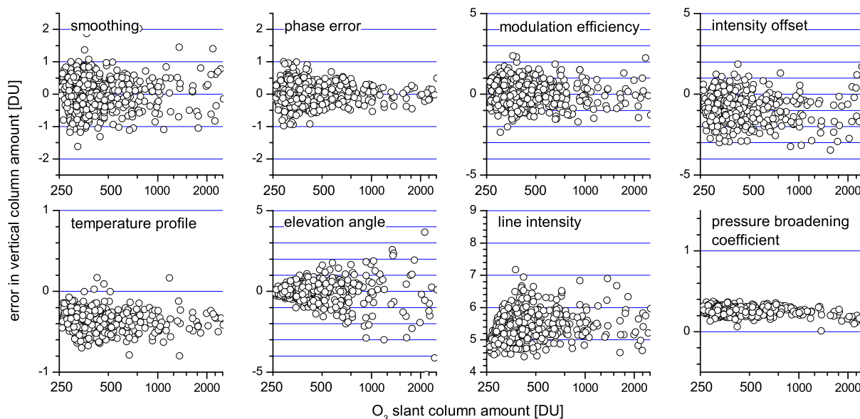
Fig. 4. Same as Fig. 2 but for new retrieval approach (i.e. simultaneous optimal estimation of O_3 and temperature profiles) and versus O_3 slant column amounts (error assumptions according to Table 1).
