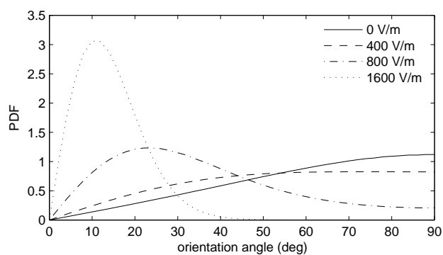
Fig. 8. Normalized probability distribution function of orientation angle of prolate ellipsoids with a long axis of 10\ \mu\text{m} , aspect ratio of 1.5 and density is 2.6\ \text{g/cm}^3 , falling under gravity and subjected to a vertical electric field (strength shown in the legend).
