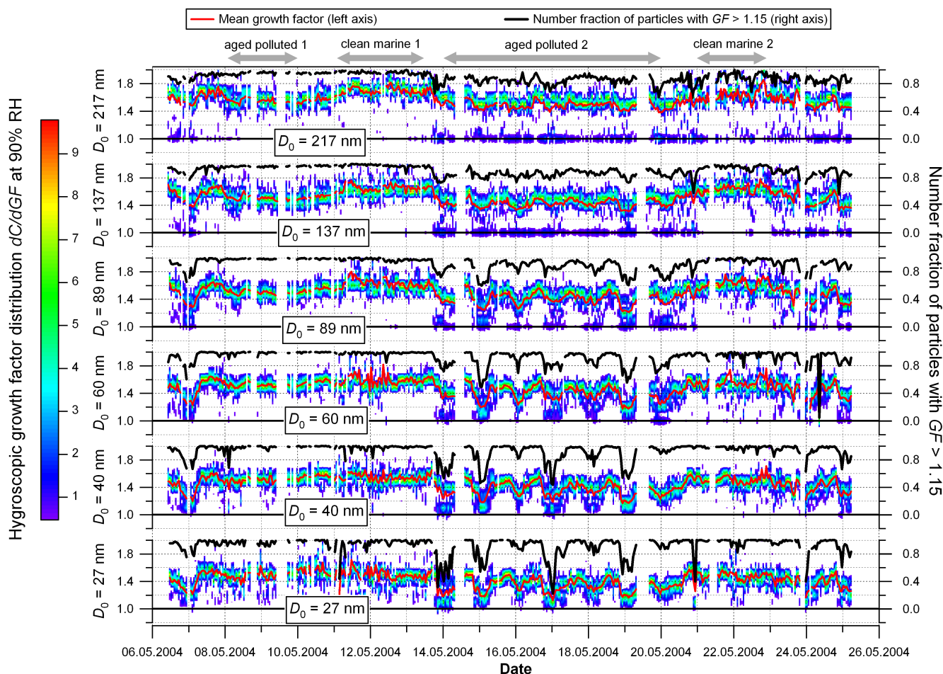
Fig. 1. Growth factor probability distributions for different particle dry sizes as measured with a HTDMA. The red lines represent the 3 rd -moment mean growth factors, black lines the number fraction of particles with g > 1.15 .
