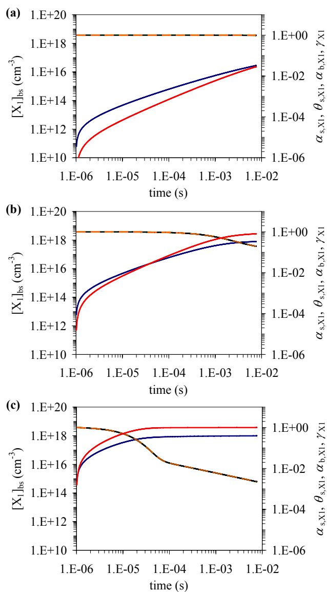
Fig. 9. Temporal evolution of sorption layer surface coverage \theta_{s,X1} (red), surface accommodation coefficient \alpha_{s,X1} (black), bulk accommodation coefficient \alpha_{b,X1} (orange), uptake coefficient \gamma_{X1} (green) and particle bulk composition (blue) in model system L2 describing adsorption and diffusion-limited surface-bulk transport of a trace gas X_1 (i.e., non-reactive solvation of a trace gas into a liquid aerosol): scenario L2-7 (a) with [X_1]_{gs}=1 \times 10^{11} cm -3 , scenario L2-8 (b) with [X_1]_{gs}=1 \times 10^{13} cm -3 and scenario L2-9 (c) with [X_1]_{gs}=1 \times 10^{15} cm -3 .
