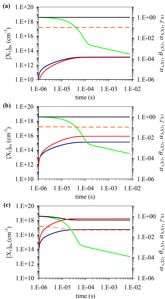
Fig. 7. Temporal evolution of sorption layer surface coverage \theta_{s,X1} (red), surface accommodation coefficient \alpha_{s,X1} (black), bulk accommodation coefficient \alpha_{b,X1} (orange), uptake coefficient \gamma_{X1} (green) and particle bulk composition (blue) in model system L2 describing adsorption and diffusion-limited surface-bulk transport of a trace gas X_1 (i.e., non-reactive solvation of a trace gas into a liquid aerosol): scenario L2-1 (a) with [X_1]_{gs}=1 \times 10^{11} \text{ cm}^{-3} , scenario L2-2 (b) with [X_1]_{gs}=1 \times 10^{13} \text{ cm}^{-3} and scenario L2-3 (c) with [X_1]_{gs}=1 \times 10^{15} \text{ cm}^{-3} . The further parameters associated with these scenarios are listed in Table 1. The temporal evolution for the other scenarios of model system L2 listed in Table 1, L2-4 to L2-6 and L2-7 to L2-9, are presented in Figures 8 and 9, respectively.
