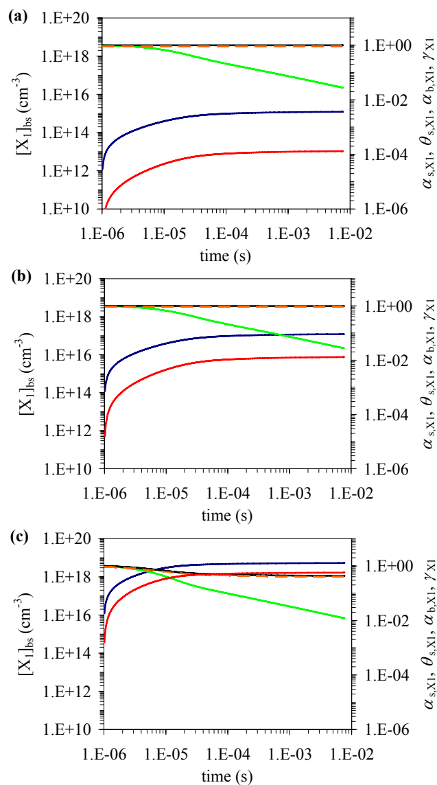
Fig. 8. Temporal evolution of sorption layer surface coverage \theta_{s,X1} (red), surface accommodation coefficient \alpha_{s,X1} (black), bulk accommodation coefficient \alpha_{b,X1} (orange), uptake coefficient \gamma_{X1} (green) and particle bulk composition (blue) in model system L2 describing adsorption and diffusion-limited surface-bulk transport of a trace gas X_1 (i.e., non-reactive solvation of a trace gas into a liquid aerosol): scenario L2-4 (a) with [X_1]_{gs}=1 \times 10^{11} \text{ cm}^{-3} , scenario L2-5 (b) with [X_1]_{gs}=1 \times 10^{13} \text{ cm}^{-3} and scenario L2-6 (c) with [X_1]_{gs}=1 \times 10^{15} \text{ cm}^{-3} .
