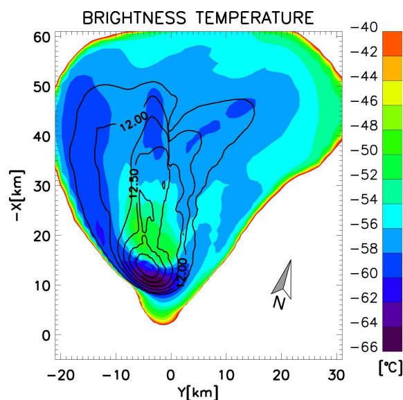
Fig. 7. Brightness temperatures derived from upwelling radiance simulated for the 10.8 \mu m wavelength band. The contour lines indicate the altitude in km of the 100 \mu g m^{-3} isosurface of the aerosol mass concentration.
