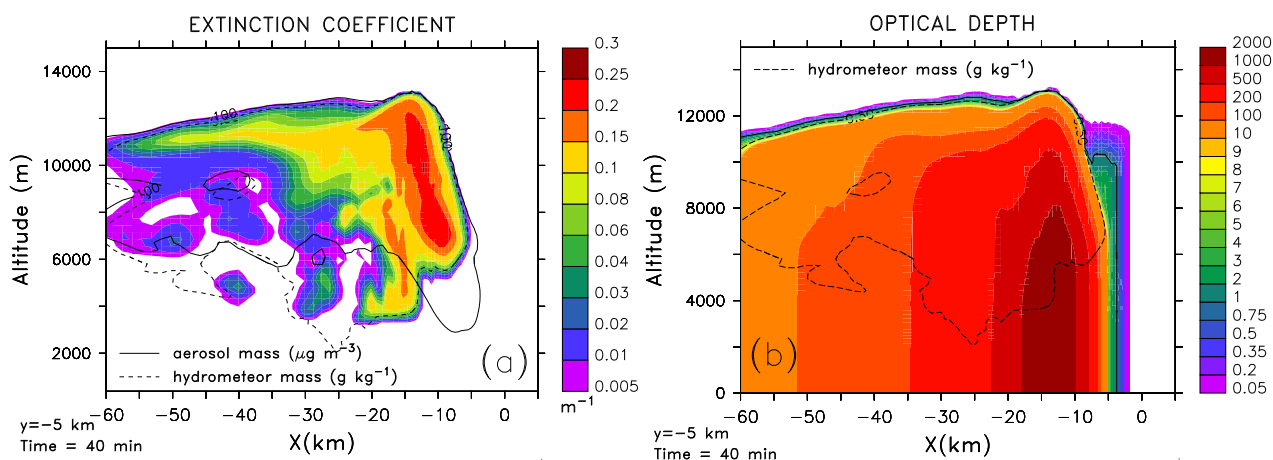
Fig. 6. Results from offline calculation of radiative properties. (a) Extinction due to absorption and scattering by hydrometeors and aerosols at 10.8 \mu m . Contours of aerosol mass concentration (solid line) and hydrometeor concentration (dashed line) indicate the extent of the smoke plume and pyroCb. (b) Aerosol and hydrometeor extinction optical depth \tau at 10.8 \mu m from the top of the atmosphere as a function of z . Note that the \tau=1 contour (solid line), which can be used as an indication of the effective level of emission of the thermal radiation, is situated very close to the cloud top.
