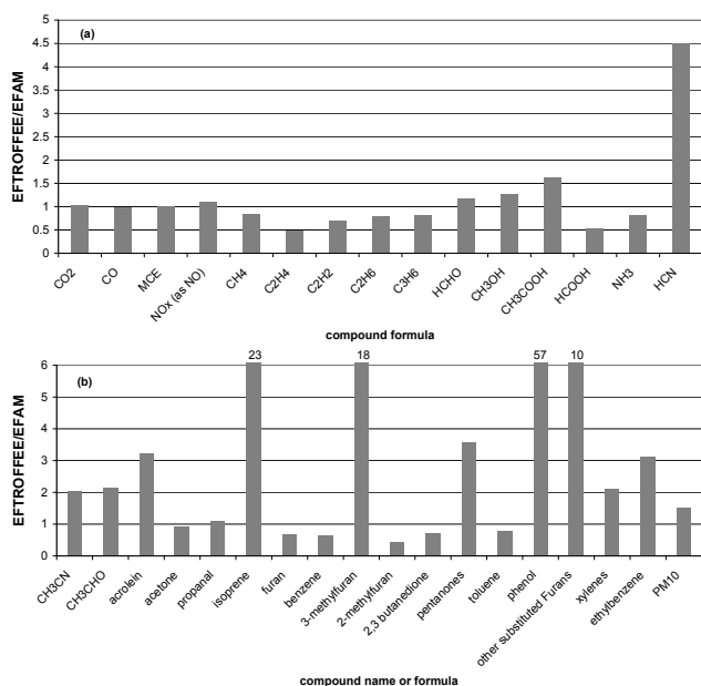
Fig. 6. Comparison of the TROFFEE airborne study emission factors with the recommendations of Andrea and Merlet (2001) (AM) for species in both studies. (AM PM_{10} is taken as 1.3 \times AM PM_{2.5} .) With 8 exceptions, the older (AM) recommendations are within a factor of \sim 2 of the newer TROFFEE EF, which are usually based on more measurements. This suggests that the AM recommendations for species not measured in TROFFEE (e.g. SO_2 ) are reasonable. (a) species measured by AFTIR. (b) species measured by PTR-MS and the nephelometer. (When the ratio exceeds the scale shown the value of the ratio is given above the bar.)
