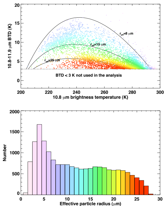
Fig. 2. Ice mass retrievals from SEVIRI 11 and 12 \mu\text{m} data. Observed 11–12 \mu\text{m} brightness temperature difference (BTD in K) vs. 11 \mu\text{m} brightness temperature (K) for 9 consecutive SEVIRI images spanning the time interval 19:30 to 21:30 UT on 20 May 2006 (top panel). The points are colour coded to show particle size; lilac represents small particles ( <8 \mu\text{m} ) and red represents larger particles ( >25 \mu\text{m} ). The effective particle size histogram for \sim 50\,000 data points is also shown (bottom panel).
