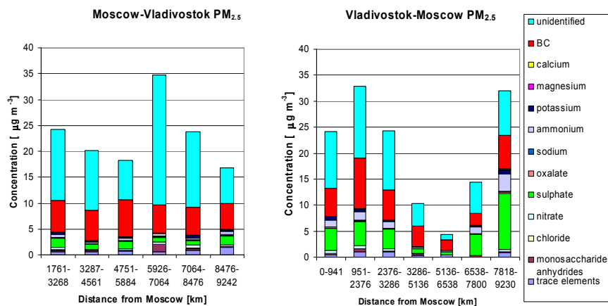
Fig. 5. The mass concentrations of ions, BC, monosaccharide anhydrides, trace elements and unidentified matter in PM_{2.5} between Moscow and Vladivostok.
