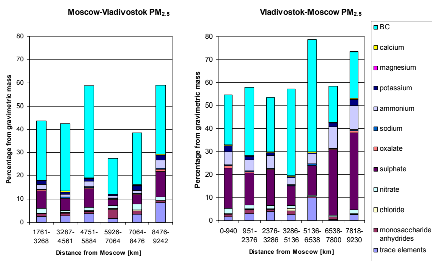
Fig. 6. The contributions of ions, BC, monosaccharide anhydrides, trace elements and unidentified matter to PM_{2.5} between Moscow and Vladivostok.
