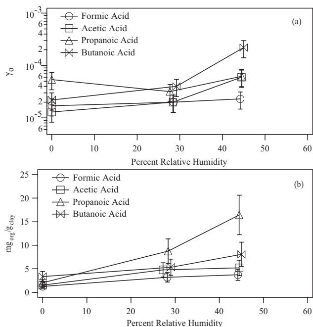
Fig. 8. (a) The initial uptake efficiencies on a log scale for the uptake of formic, acetic, propanoic and butanoic acids on approximately 1.5 mg SWy-2 at 1.3 \times 10^{-4} hPa organic acid pressure, 1.3 \times 10^{-5} hPa butanoic acid and 212 K as a function of RH. (b) The organic acid content, \text{mg}_{\text{org}}/\text{g}_{\text{clay}} , of adsorbed formic, acetic, propanoic and butanoic acids on approximately 1.5 mg SWy-2 at 212 K as a function of RH. Lines are drawn to guide the eye.
