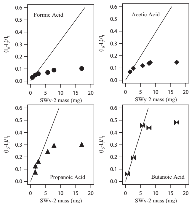
Fig. 5. (I_o - I_t)/I_t obtained from organic acid uptake measurements at 212 K and 29% RH as a function of SWy-2 mass after two seconds of exposure. Formic, acetic and propanoic acid uptake experiments were performed in the presence of approximately 1.3 \times 10^{-4} hPa acid while butanoic acid uptake measurements were performed in the presence of approximately 1.3 \times 10^{-5} hPa butanoic acid.
