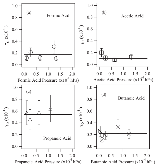
Fig. 6. Initial uptake efficiencies for (a) formic, (b) acetic, (c) propanoic and (d) butanoic acid uptake on approximately 1.5 mg SWy-2 at 212 K and 0% RH as a function of organic acid pressure. The horizontal lines represent the average \gamma_o value obtained over the range of partial pressures studied.
