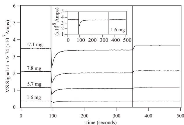
Fig. 4. Raw uptake curves of propanoic acid on 1.6, 5.7, 7.8 and 17.1 mg SWy-2 samples at 212 K, 29% RH and approximately 1.3 \times 10^{-4} hPa propanoic acid. The inset shows an expanded view of the propanoic acid uptake curve on the 1.6 mg SWy-2 clay sample. The vertical lines represent the time SWy-2 was exposed to the gas phase. The traces are offset for clarity.
