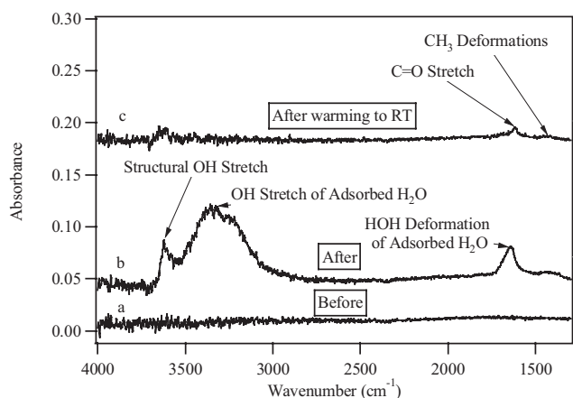
Fig. 2. FT-IR spectra collected (a) before and (b) after exposure of a 1.2 mg SWy-2 sample to 1.3 \times 10^{-4} hPa acetic acid at 212 K and 29% RH. (c) Also shown is the infrared spectrum collected after warming the sample to room temperature to drive off adsorbed water. All spectra are ratioed to a background spectrum of the clay collected prior to exposure at the same temperature.
