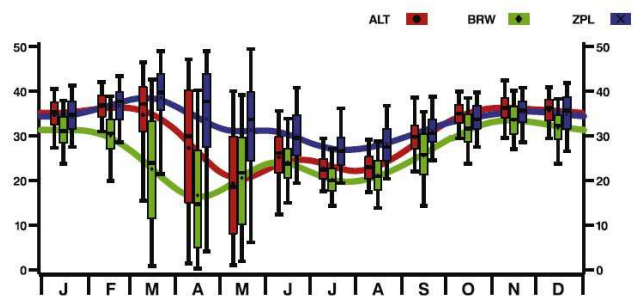
Fig. 1. Box and whisker plots showing 9 years of observations of O_3 mole fractions (in nmol/mol) at Alert (red), Barrow (green), and Zeppelinfjället (also called Ny-Ålesund in this paper) (blue). The smoothing curves were generated by LOWESS, a nonparametric technique used here to illustrate the seasonal cycles for the three stations (Cleveland and Devlin, 1988; Peña et al., 2000). Lower and upper whiskers are the 5th and 95th percentiles, while the bottom and top of boxes are the 25th and 75th percentiles, respectively. Horizontal lines inside the boxes are monthly median values for the 9-year period, and the symbols are monthly means. Reprinted from Bottenheim and Chan (2006) with permission from the American Geophysical Union (AGU).
