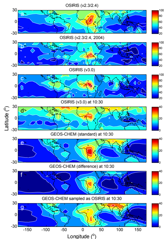
Fig. 4. (a) OSIRIS operational NO 2 VMR (v2.3/2.4) at 12 km, in pmol/mol; AM data only, averaged over all available data and gridded on 8^\circ \times 10^\circ (latitude, longitude), (b) same as (a), but for the year 2004, (c) same as (a) but for v3.0, (d) same as (c), but with diurnal scaling to 10:30 LT and with stratospheric points removed by defining the tropopause (see McLinden et al., 2000) as the lowest altitude with 150 nmol/mol of OSIRIS O 3 (v3.0), (e) map of annual mean NO 2 VMR including lightning at z=12 km for the year 2000, calculated for 10:30 LT with the GEOS-Chem model. (f) same as (e) except the difference is taken from a model run without lightning to isolate the contribution from lightning, (g) same as (e), except that, an attempt was made to match the spatiotemporal sampling of GEOS-Chem with that of OSIRIS. The monthly mean model data was weighted by the fraction of all OSIRIS data points that occurred in that month in order to make the temporal sampling of GEOS-Chem consistent with that of OSIRIS. The weighting according to the temporal measurement frequency of OSIRIS is performed as a function of latitude.
