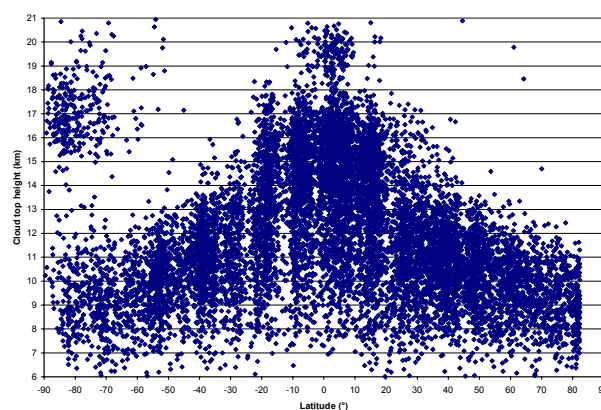
Fig. 1. Cloud top heights observed by OSIRIS from \sim 1100 selected orbits during the period of investigation (27 May 2003–27 May 2005). Orbits are included from each month. Polar stratospheric clouds are observed in austral spring at high latitudes at \sim 17 km.
