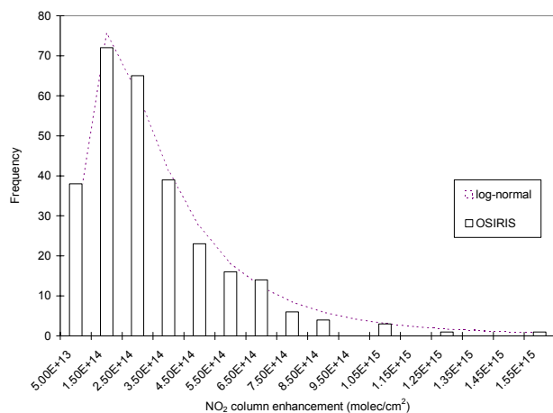
Fig. 7. Distribution of OSIRIS UT NO 2 column enhancements due to lightning is well described ( r^2=0.9754 ) by a 3-parameter log-normal distribution. Bin midpoint values are labeled along the x-axis. No effort has been made to scale column enhancements to a single local time.
