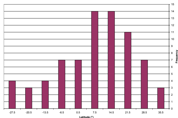
Fig. 6. Histogram of OSIRIS UT NO 2 enhancements detected over Africa over the 2 year period (May 2003–May 2005). The latitude at the midpoint of each bin is labeled on the x-axis.
