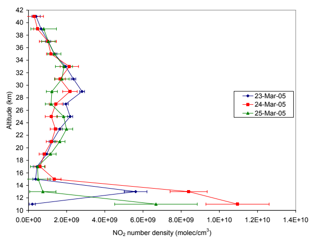
Fig. 9e. NO 2 number density profiles observed by OSIRIS at 32.3^\circ N, 58.7^\circ W on 23/03/2005 (SZA= 89.643^\circ PM), at 27.3^\circ N, 46.4^\circ W on 24 March 2005 (SZA= 80.746^\circ AM), and at 27.7^\circ N, 0.3^\circ E on 25 March 2005 (SZA= 80.563^\circ AM). The profiles on 24–25 March 2005 have been scaled to SZA= 89.643^\circ PM to allow for comparison of the profiles without diurnal differences in NO x partitioning.
