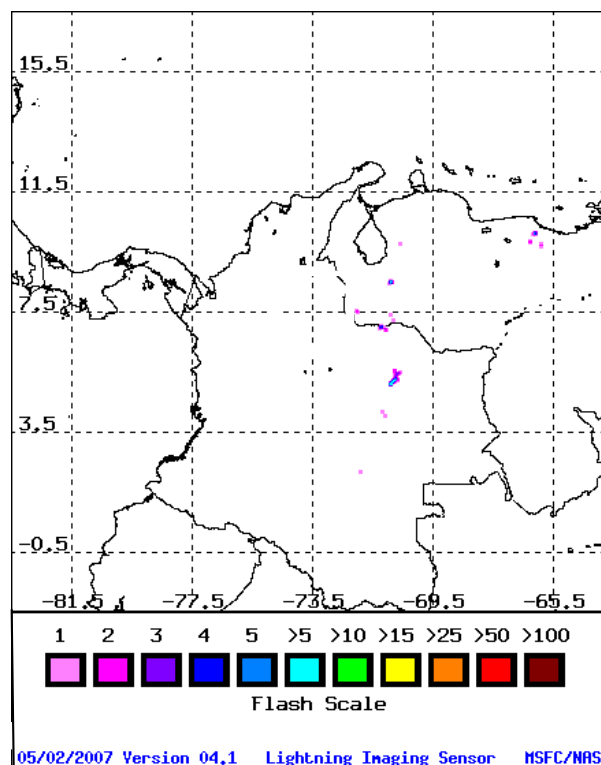
Fig. 10b. Map of lightning flashes from LIS over Colombia on 5 August 2004 between 06:13 and 08:01 UTC.
