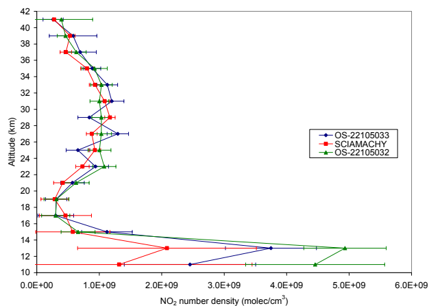
Fig. 8a. Comparison of NO 2 profiles from SCIAMACHY (25.923° S, 76.002° E, SZA=44° AM) and OSIRIS on 15/03/2005 after nearby lightning flashes hours earlier led to large enhancements in NO 2 . OSIRIS scans 32 and 33 are at (27.22° S, 76.1° E, SZA=88.09° AM) and (27.949° S, 76.0° E, SZA=88.59° AM), respectively, for TH \approx 13 km. All three profiles have been converted to SZA=88.59° AM to account for diurnal variation using a photochemical model (McLinden et al., 2000; see also Brohede et al., 2007).
