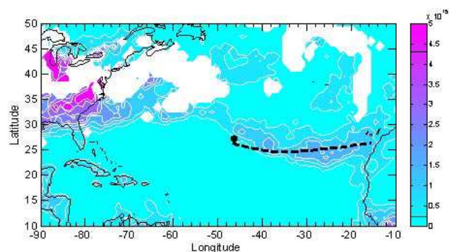
Fig. 9d. Same as (c), except for 24 March 2005. OMI data was not available on 25/03/2005 for the Atlantic region.
