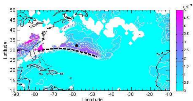
Fig. 9c. Tropospheric column NO 2 (molec/cm 2 ) from OMI on 23 March 2005 showing a plume of NO 2 transported along the trajectory starting at 02:00 UTC on 23 March 2005, also shown in Fig. 9b. The trajectory during the same calendar day (UTC) is shown. The filled black circle represents the location of the OSIRIS profile from the same calendar day (shown below). Cloudy OMI data have been filtered using a cloud fraction threshold of 0.5. The local time of the OMI measurements is approximately 13:30.
