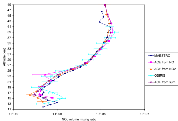
Fig. 10a. Coincident profiles of NO x inferred from measurements of NO or NO 2 observed by three satellite instruments on 06/08/2004 showing enhanced mixing ratios in the upper troposphere shortly after several nearby lightning strikes in tropical South America. MAESTRO and ACE observed NO 2 while the latter also observed NO at local sunset (3.3° N, 71.7° W). OSIRIS (2° N, 71° N) measured NO 2 just after local sunrise (SZA=85.4°). The NO x profile has been inferred by appropriately scaling by the NO x /NO or NO x /NO 2 ratio from photochemical model calculations (McLinden et al., 2000) with NO x defined here only as NO + NO 2 + 2 N 2 O 5 to account for the diurnal dissociation of N 2 O 5 . The curve “ACE from sum” is the NO x calculated by summation and the error bars reflect the quadrature sum of the uncertainties of the three species. For all other curves, uncertainties only reflect the precision of the measured species.
