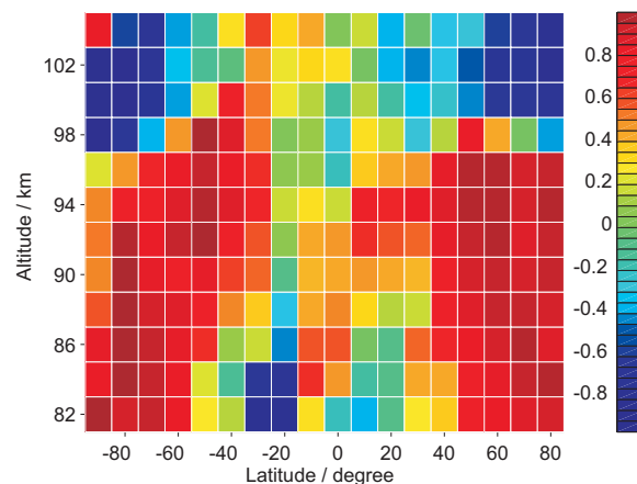
Fig. 2. Grid plot of the correlation coefficient between the NRLMSISE-00 model temperature (Picone et al., 2002) and the retrieved Na density, versus latitude and altitude.
