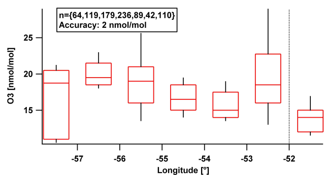
Fig. 3. Longitude profile of the O 3 median mixing ratio in the altitude range 0–1 km a.s.l.; as Fig. 2.
