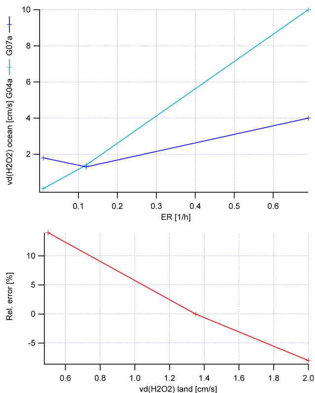
Fig. 10. Upper panel: Dependency of the derived optimum dry deposition velocity v_d(\text{H}_2\text{O}_2) over the ocean on the entrainment rate derived with the steady state box model runs for cases G04a (light blue) and G07a (dark blue). Lower panel: Relative error of the Lagrangian model result for \text{H}_2\text{O}_2 compared to the measurements versus the dry deposition velocity.
