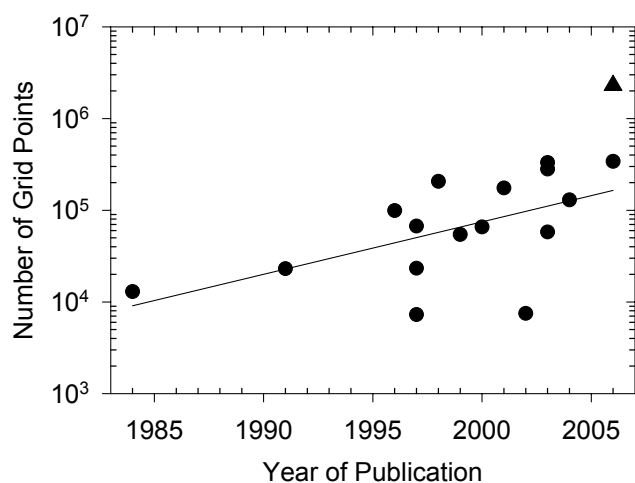
Fig. 26. Growth of numerical resolution in models versus year of publication (based on Table 12). The dots indicate the number of grid points in individual 3-D numerical models, the line represents a linear regression. The triangle denotes the number of grid points in the ECMWF forecast model which is operational since 2006.
