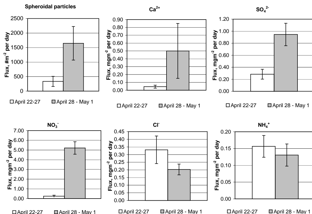
Fig. 5. Average deposition fluxes with error bars of inorganic compounds and spheroidal particles of two sampling periods during the LAPBIAT measurement campaign, in # m -2 per day for spheroidal particles and mg m -2 per day for other species. The fluxes are based on snow samples that were collected from several locations close to SMEAR I station.
