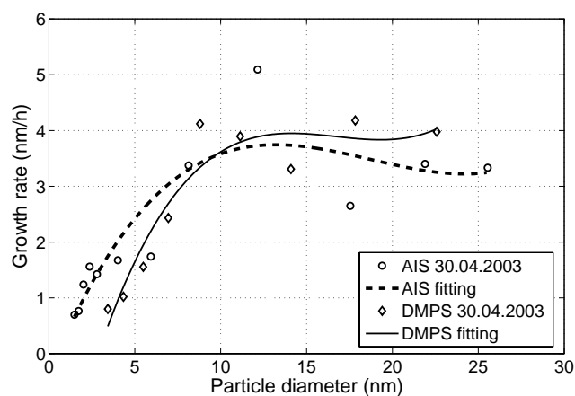
Fig. 10. The new particle and air ion growth rates as a function of size on 30 April 2003 at SMEAR I station.
