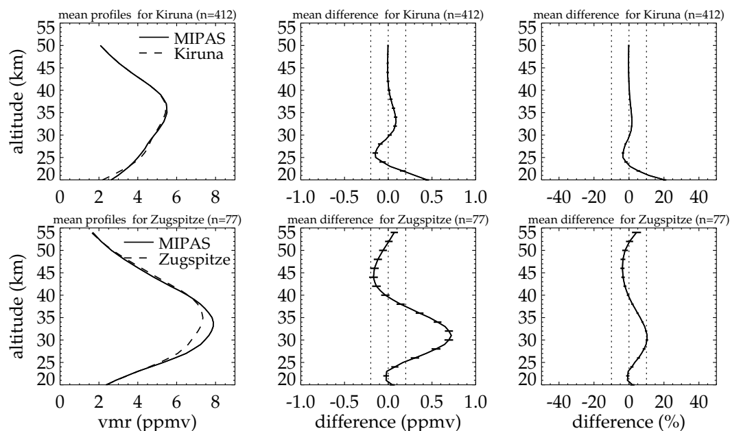
Fig. 7. Comparison of MIPAS and microwave ozone profiles. From top to bottom (number of coincidences in brackets): Kiruna (412) and Zugspitze (77). From left to right: see Fig. 5.
