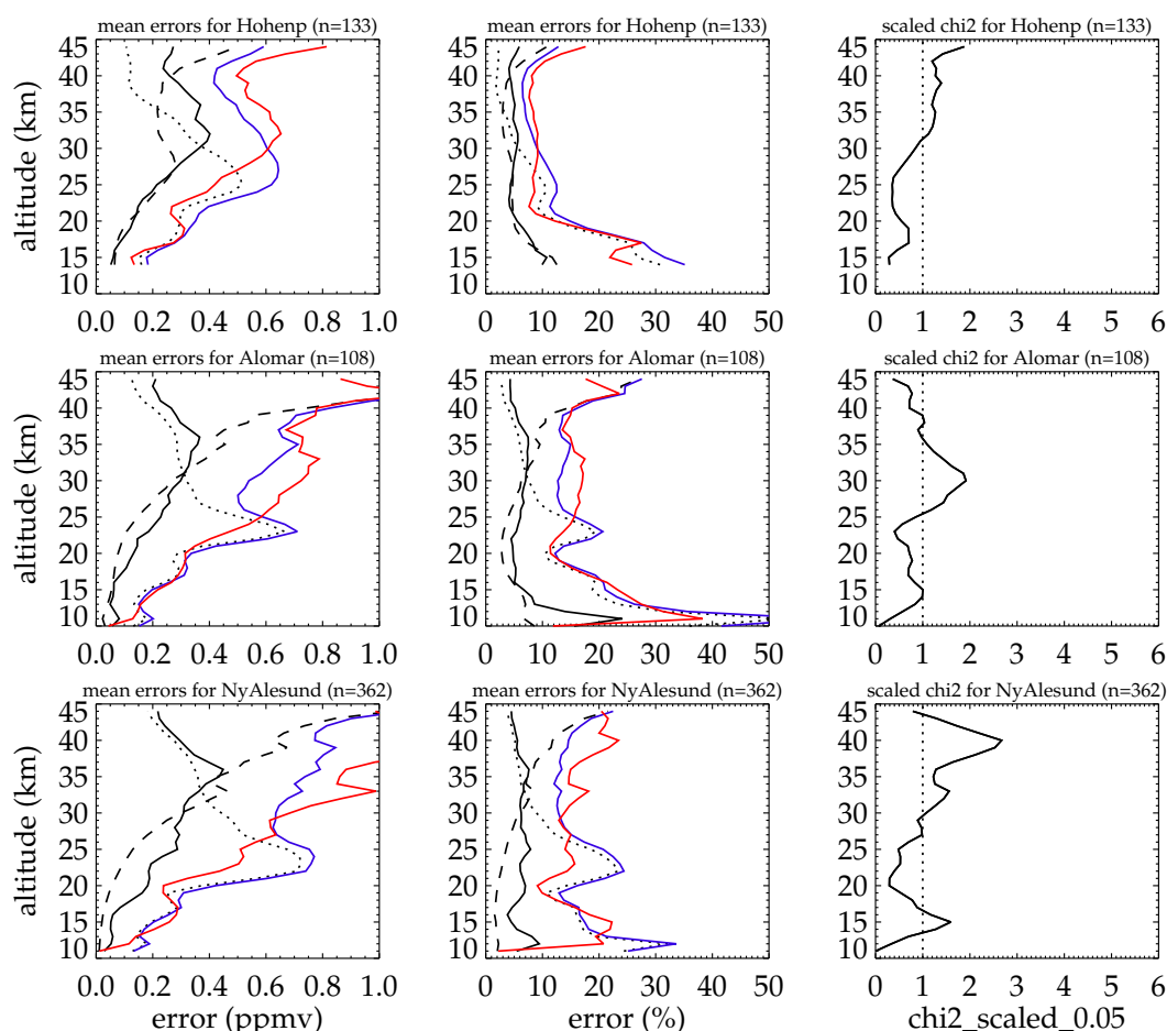
Fig. 14. Analysis of MIPAS and lidar ozone random errors. From top to bottom (number of coincidences in brackets): Hohenpeissenberg (133), Alomar (108), and Ny-Ålesund (362). From left to right: mean absolute errors (solid: MIPAS random, dashed: lidar random, dotted: mismatch, blue: combined random, red: de-biased rms difference), percentage mean errors (lines as for absolute errors), and scaled \chi^2 values (dotted line marks the 95% limit).
