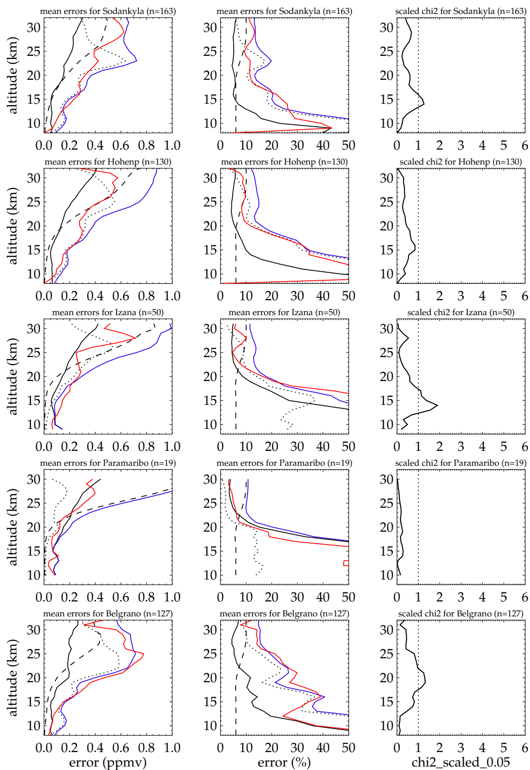
Fig. 17. Analysis of MIPAS and ozonesonde random errors. From top to bottom (number of coincidences in brackets): Sodankyla (163), Hohentpeissenberg (130), Izana (50), Paramaribo (19), and Belgrano (127). From left to right: see Fig. 14.
