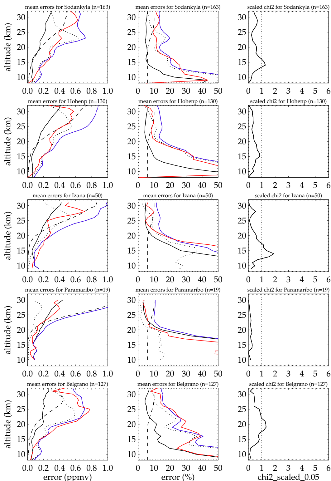
Fig. 17. Analysis of MIPAS and ozonesonde random errors. From top to bottom (number of coincidences in brackets): Sodankyla (163), Hohenpeissenberg (130), Izana (50), Paramaribo (19), and Belgrano (127). From left to right: see Fig. 14.
