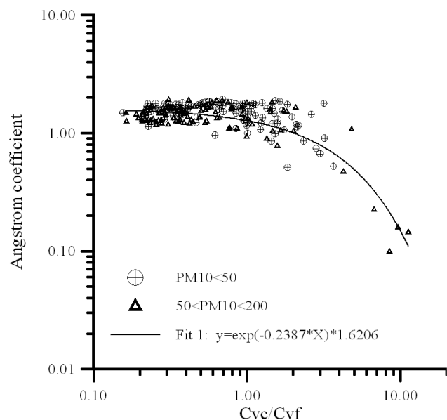
Fig. 11. Ångström coefficient versus C_{vc}/C_{vf} for clean days (PM 10 <50 \mu\text{g}/\text{m}^3 ) and with moderate smog (50≤PM 10 <200 \mu\text{g}/\text{m}^3 ). The exponential fit is obtained for data points (N=105) representing days with moderate smog. The correlation coefficient is 0.798.
