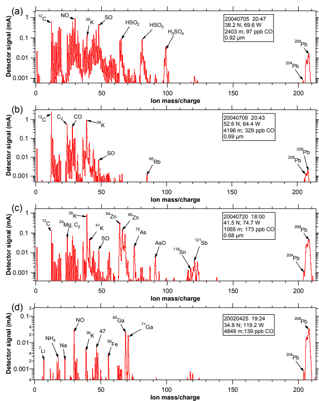
Fig. 4. Examples of mass spectra of single particles containing Pb. (a) A common mixed sulfate-organic particle. (b) A particle in a biomass burning plume over Canada. (c) A particle with other metals. The association of Pb with one or more of K, Zn, Sn, and Sb was common. (d) A Pb-Ga particle from trans-Pacific flow west of California. Gallium is quite rare in atmospheric particles, but the isotopic pattern is definitive.
