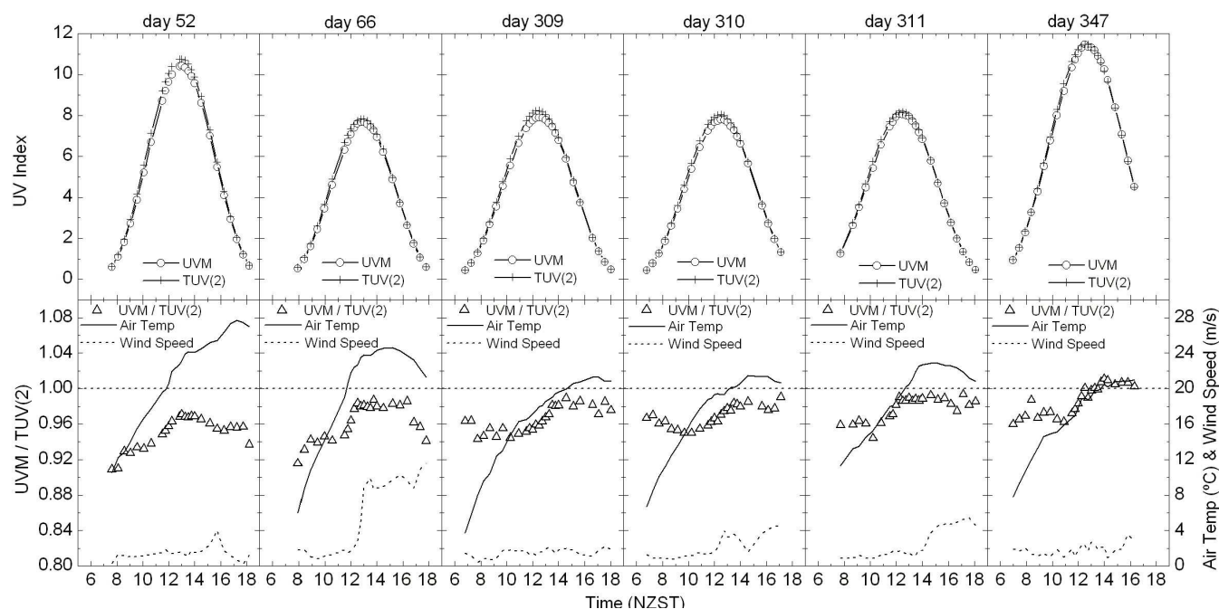
Fig. 11. UVI model vs. measurement comparison for six days of 2001 in Lauder for which air temperature clearly exceeded 20°C and diurnal variations in TOZ and AOD were small. Upper: Measured (circles) and modelled (crosses) UVI as a function of time. Lower: Measured over modelled UVI ratio (triangles), air temperature (solid line) and wind speed (dashed line) as a function of time.
