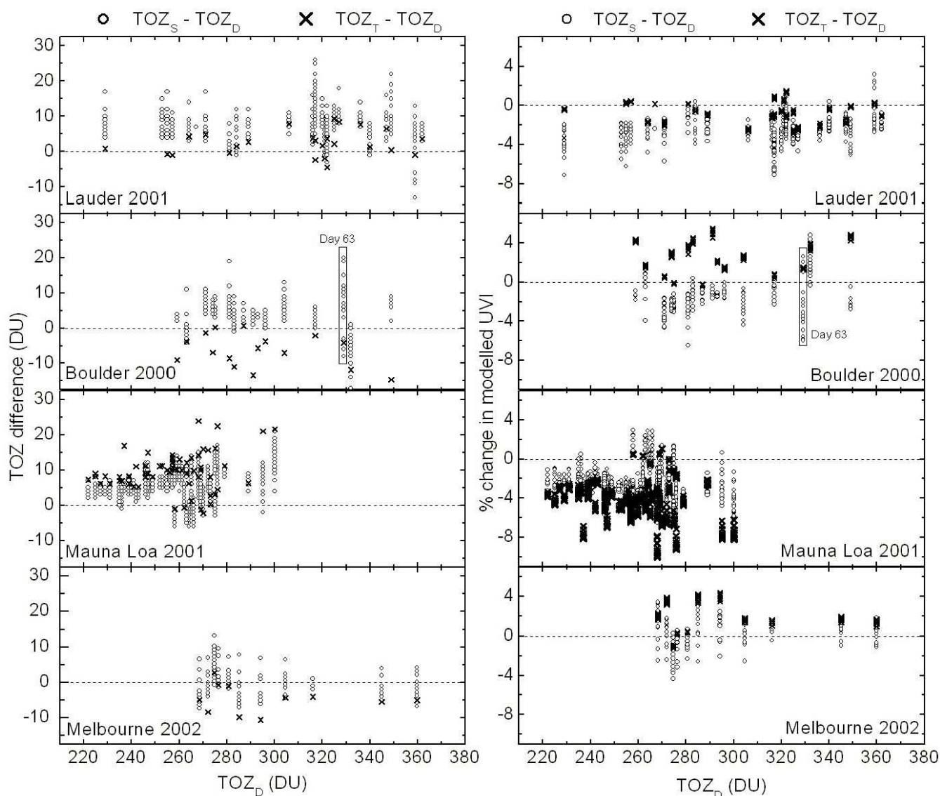
Fig. 2. Left panel: Differences in ozone measurements: \text{TOZ}_T - \text{TOZ}_D (crosses) and \text{TOZ}_S - \text{TOZ}_D (circles) in DU for the datasets in Fig. 1. Right Panel: Relative differences (in %) in calculated UVI from using \text{TOZ}_T (crosses) and \text{TOZ}_S (circles) instead of \text{TOZ}_D as input to the model.
