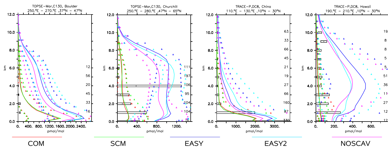
Fig. 13. As Fig. 7, but for SO 2 .
