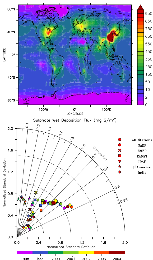
Fig. 3. Average annually accumulated wet deposition of sulphate in \text{mg S/m}^2 (upper panel) and comparison with observations in a Taylor diagram (lower panel). For the notation see Fig. 2.
