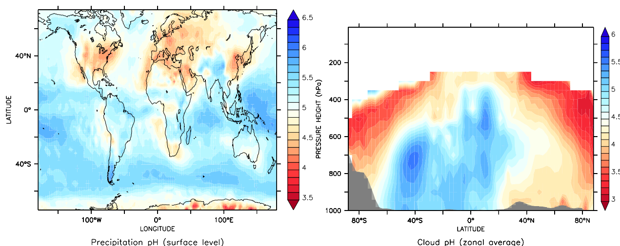
Fig. 5. Annual average precipitation pH at the surface from large-scale and convective precipitation (left) and annual zonal average of the cloud pH (right).
