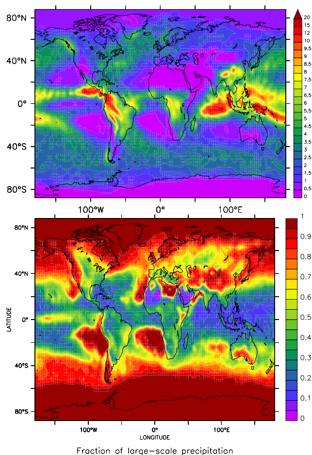
Fig. 1. Annual average precipitation rate in mm/day of the EVAL S1 (Jöckel et al., 2006) simulation (upper panel) and fraction of the large-scale to the total precipitation (lower panel).
