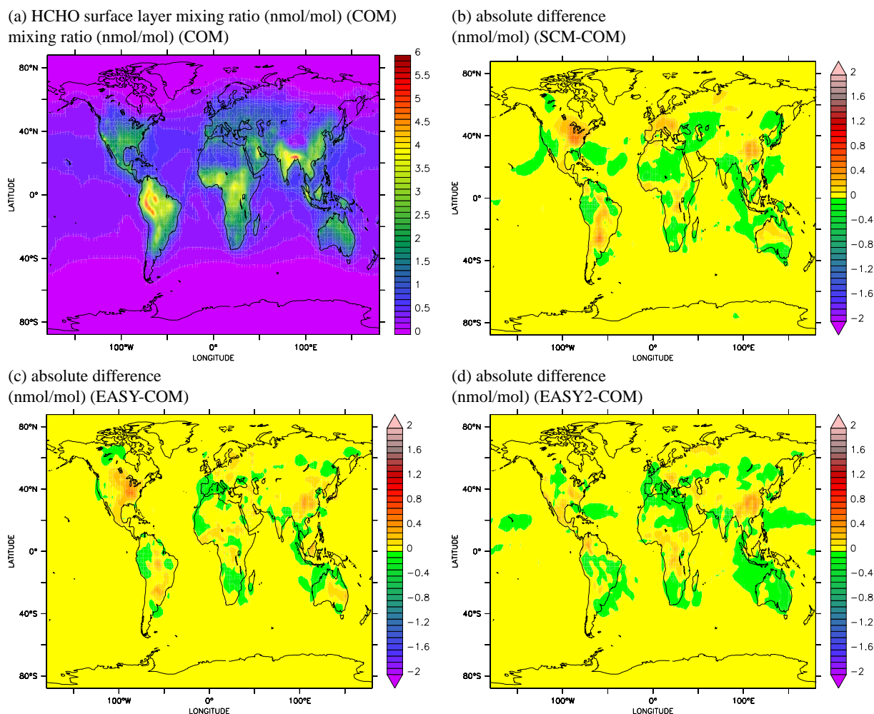
Fig. 14. Comparison of the annual average HCHO surface layer mixing ratio for the four sensitivity simulations, displayed similarly as in Fig. 6.
