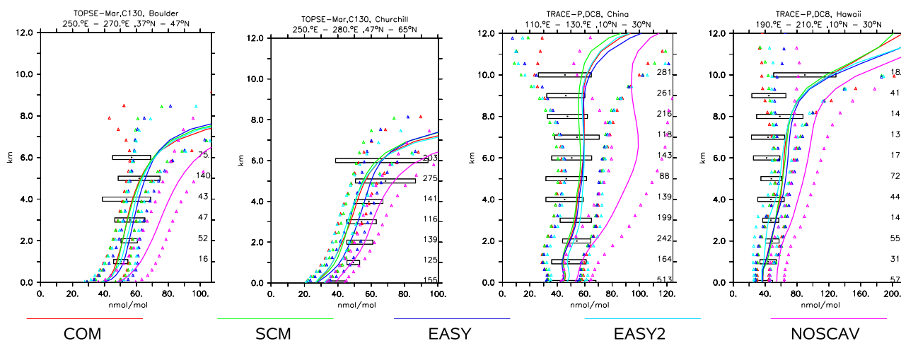
Fig. 9. As Fig. 7, but for O 3 .
