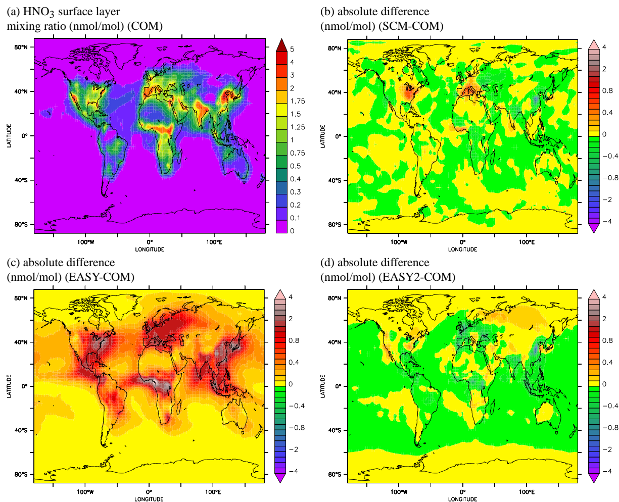
Fig. 6. Comparison of the annual average \text{HNO}_3 surface layer mixing ratio for the four sensitivity simulations: shown is the absolute value for the COM simulation (upper left panel) and – as indicated – the absolute differences of the other simulations to the COM simulation.
