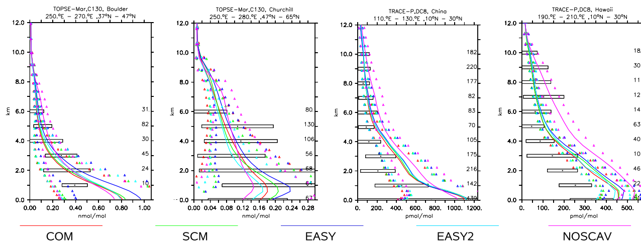
Fig. 15. As Fig. 7, but for HCHO.
