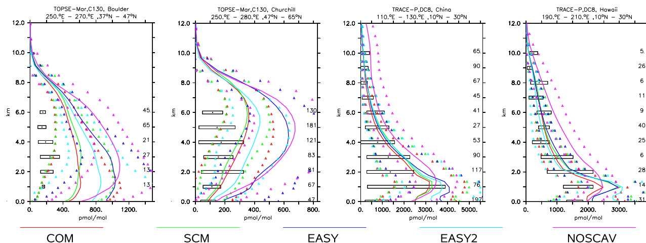
Fig. 11. As Fig. 7, but for \text{H}_2\text{O}_2 .
