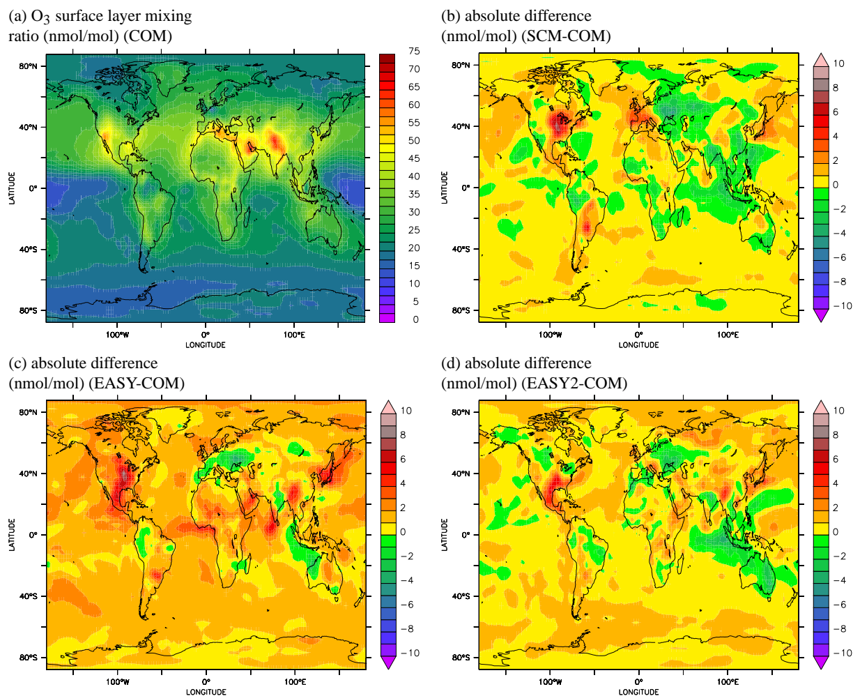
Fig. 8. Comparison of the annual average O 3 surface layer mixing ratio for the four sensitivity simulations, displayed similarly as in Fig. 6.
