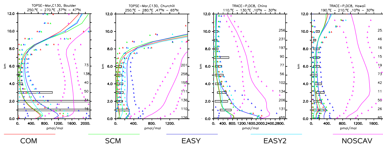
Fig. 7. Comparison of the \text{HNO}_3 vertical profiles compiled by Emmons et al. (2000) with the results of the five sensitivity simulations. The observations are depicted by the black points, their variability (standard deviation) by the black boxes and the number of points taken into account for this campaign (in space and time for this region) are listed at the right axis. The model results are represented by the solid lines and the respective standard variation by the triangles. The colours denote the simulations as indicated in the legend, i.e., red = COM, green = SCM, blue = EASY, turquoise = EASY2 and magenta = NOSCAV.
