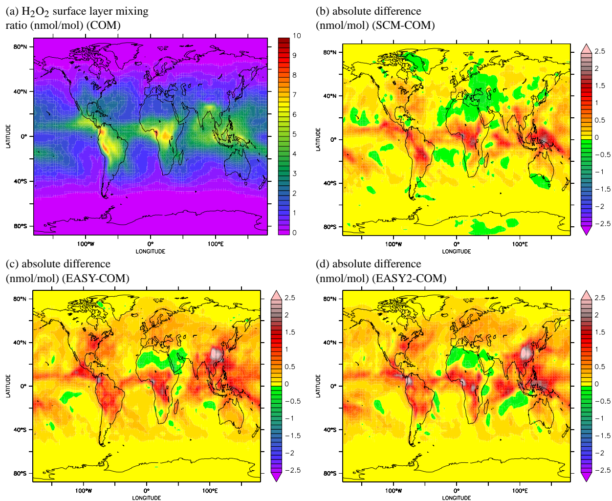
Fig. 10. Comparison of the annual average \text{H}_2\text{O}_2 surface layer mixing ratio for the four sensitivity simulations, displayed similarly as in Fig. 6.
