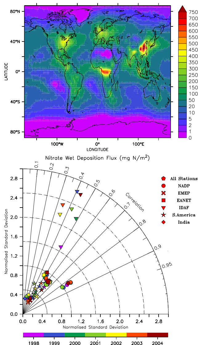
Fig. 2. Average annually accumulated wet deposition of nitrate in mg N/m 2 (upper panel) and comparison with observations in a Taylor diagram (lower panel) showing the correlation and the standard deviation of the model normalised to the standard deviation of the observations. The individual years of the simulation (colour coded) are each compared with the measurement data set. The symbols denote the different measurement networks and the composite of all observations (pentagons).
