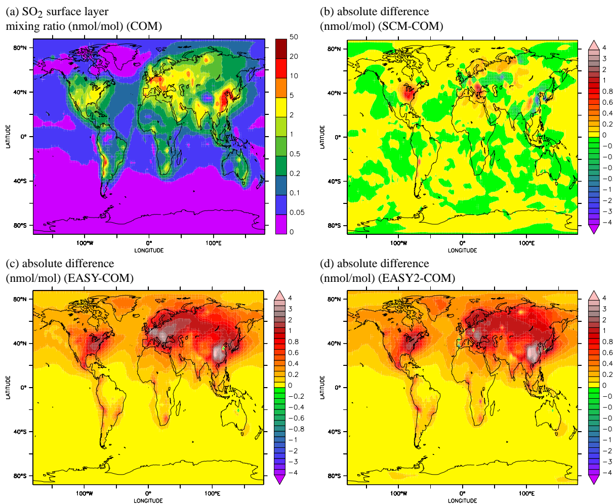
Fig. 12. Comparison of the annual average SO 2 surface layer mixing ratio for the four sensitivity simulations, displayed similarly as in Fig. 6.
