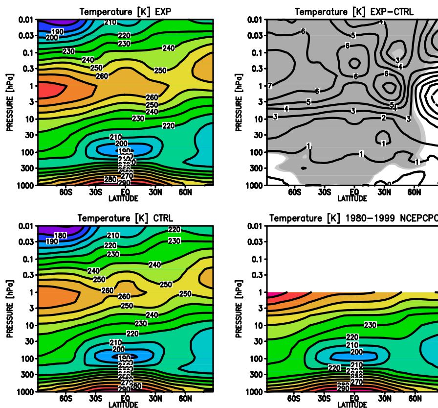
Fig. 4. January zonal mean temperature (K): (top left) for the EXP simulation; (top right) for the EXP-CTRL difference; (bottom left) for the CTRL simulation; and (bottom right) for the NCEPCPC analysis. Contour intervals is 1 K for the top right panel, and 10 K for the other three panels. For the top right panel, light and dark grey shades indicate statistical significance at the 95% and 99% levels, respectively.
